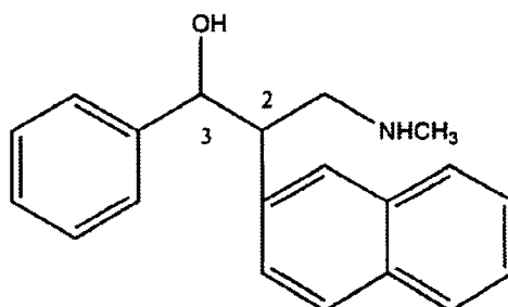
N -methyl-3-hydroxy-2-(2'-naphthyl)-3-phenylpropylamine
