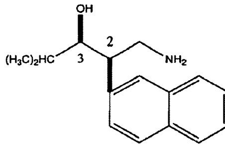
(2R,3R)-3-hydroxy-4-methyl-2-(2'-naphthyl)pentylamine
