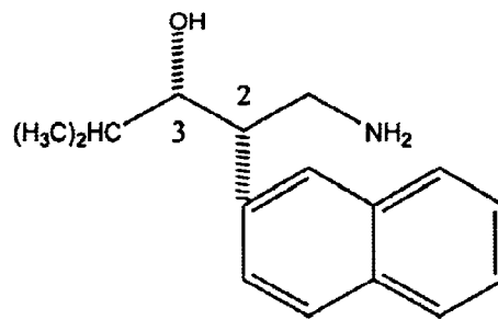
(2S,3S)-3-hydroxy-4-methyl-2-(2'-naphthyl)pentylamine
