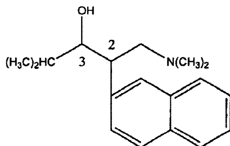
N,N -dimethyl-3-hydroxy-4-methyl-2-(2'-naphthyl)pentylamine
