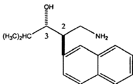
(2R,3S)-3-hydroxy-4-methyl-2-(2'-naphthyl)pentylamine
