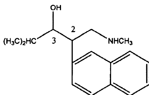
N -methyl-3-hydroxy-4-methyl-2-(2'-naphthyl)pentylamine
