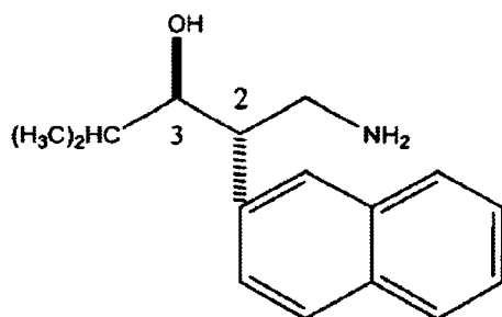
(2S,3R)-3-hydroxy-4-methyl-2-(2'-naphthyl)pentylamine
