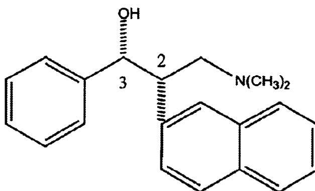
(2 S ,3 R )- N,N -dimethyl-3-hydroxy-2-(2'-naphthyl)-3-phenylpropylamine
