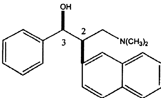
(2 R ,3 S )- N,N -dimethyl-3-hydroxy-2-(2'-naphthyl)-3-phenylpropylamine
