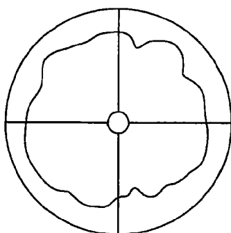
The first frequency band mode
