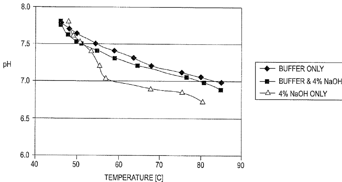
pH TEMPERATURE PROFILES DURING RAMP
