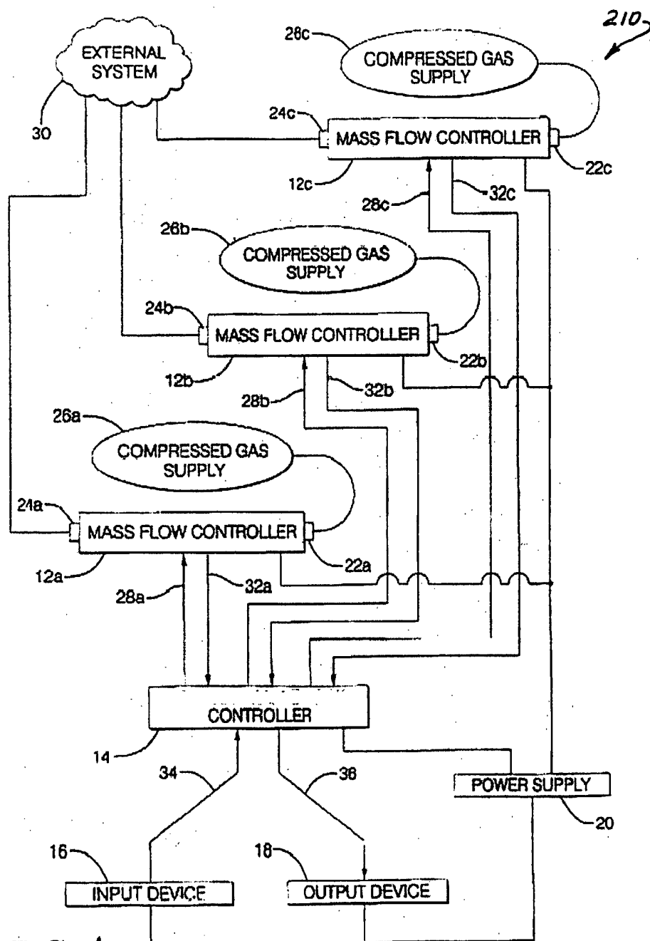
FIG. 4 (PRIOR ART)
