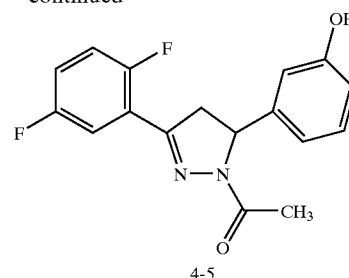
3-[1-acetyl-3-(2,5-difluorophenyl)-4,5-dihydro-1H-pyrazol-5-yl]phenyl (4-5)
