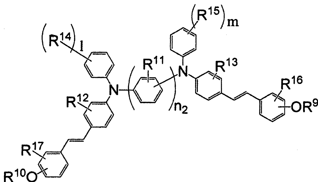
[Chem.3]
