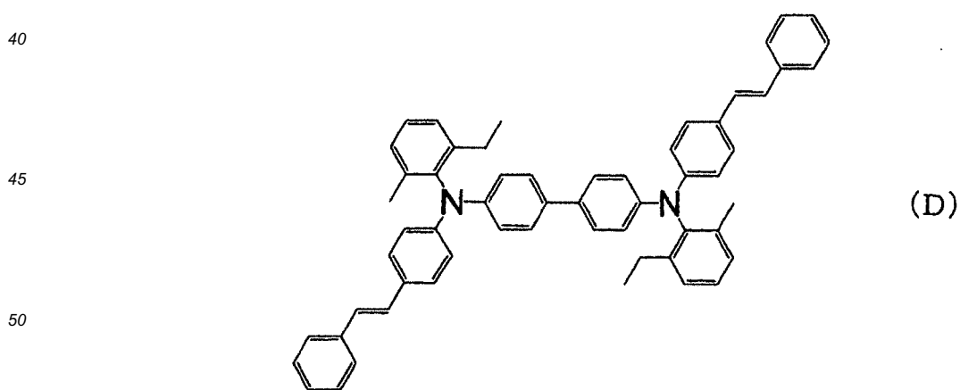
[Chem. 47]
