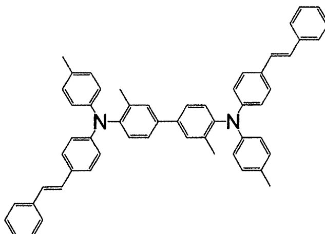
[Chem. 48]
