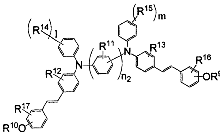
[Chem. 13]
