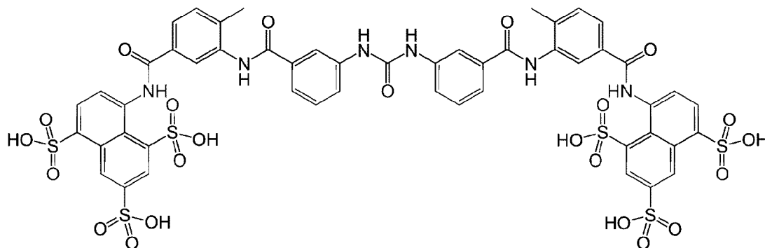
Suramin
