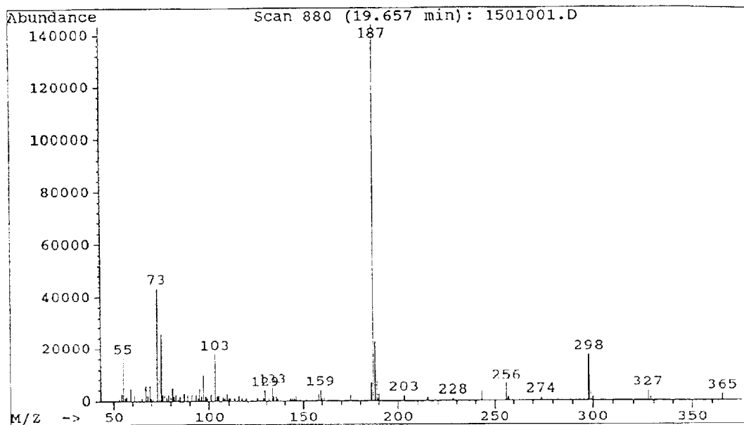
Mass spectrum of peak 12 from figure 3B
