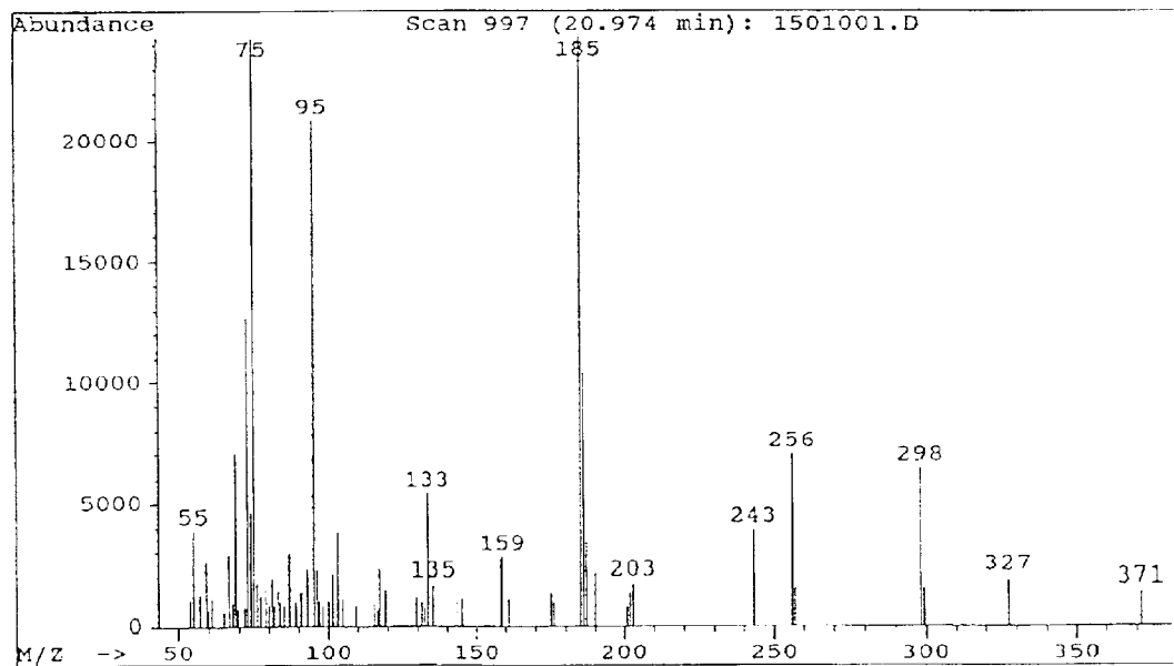
Mass spectrum of peak 13 from figure 3B
