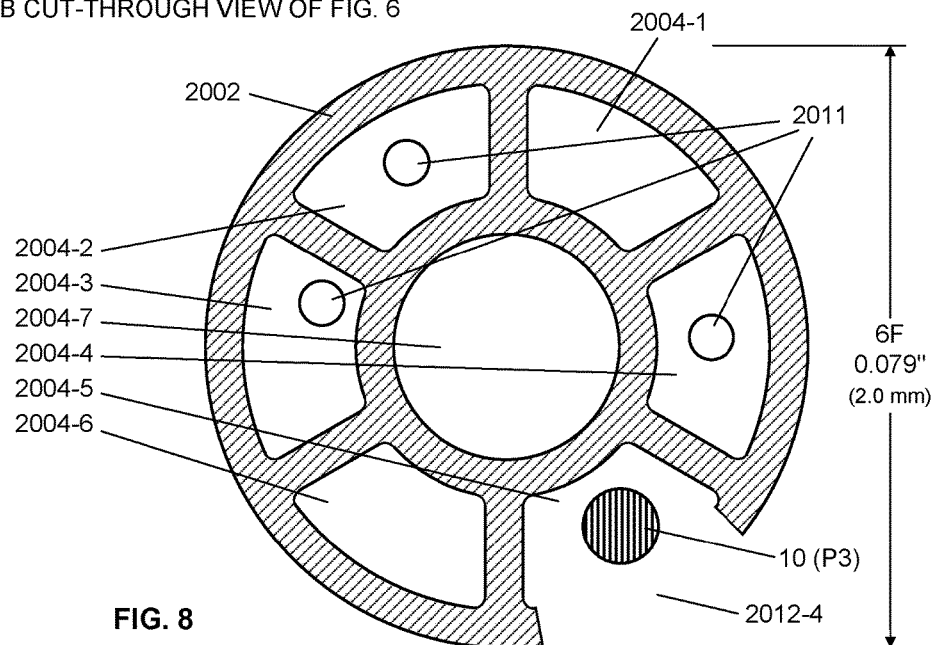
B-B CUT-THROUGH VIEW OF FIG. 6
