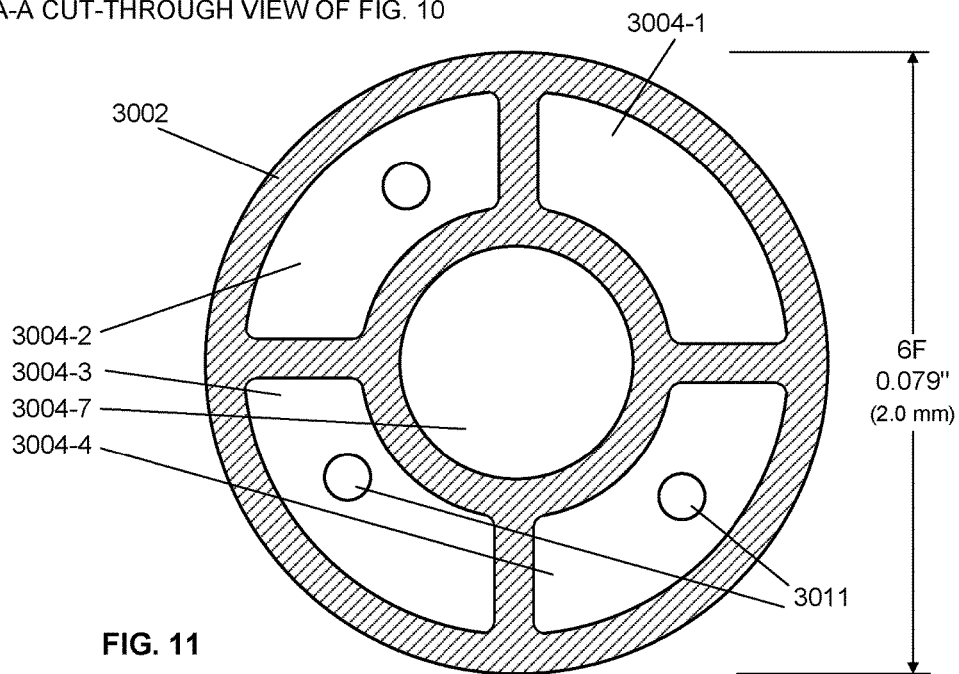
A-A CUT-THROUGH VIEW OF FIG. 10
