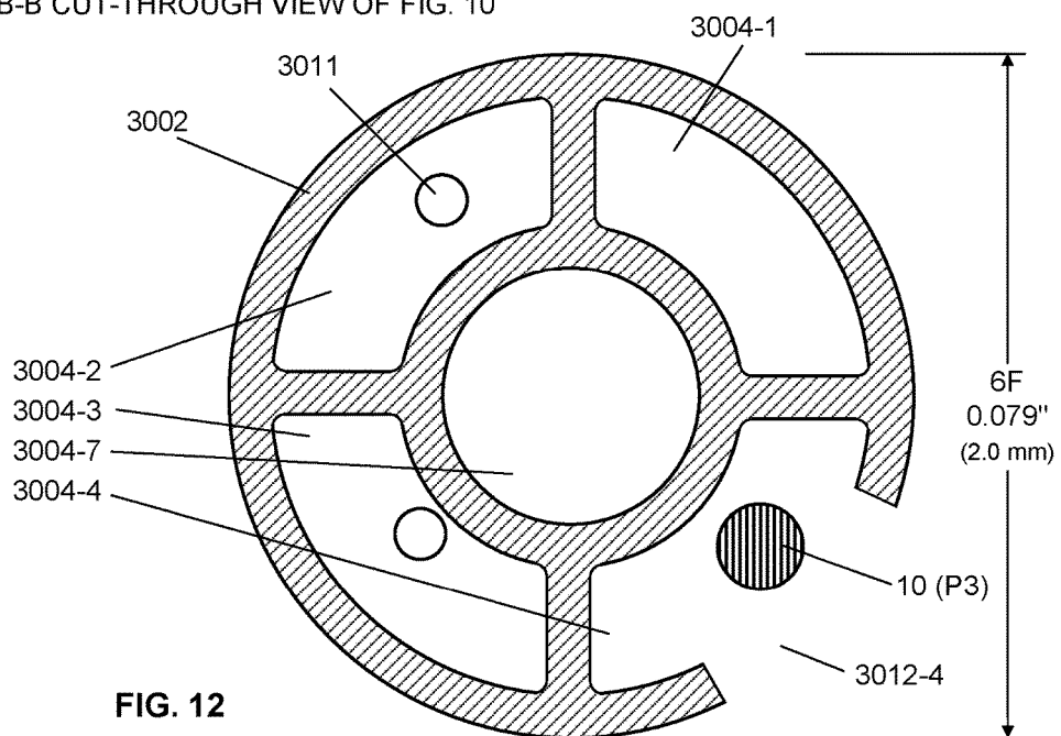
B-B CUT-THROUGH VIEW OF FIG. 10
