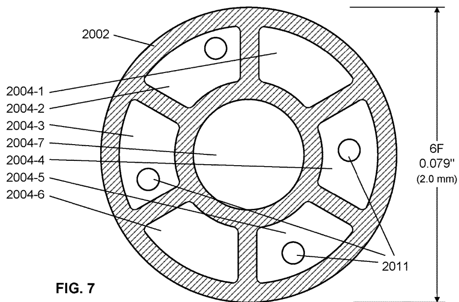
A-A CUT-THROUGH VIEW OF FIGS. 5, 6 AND 9
