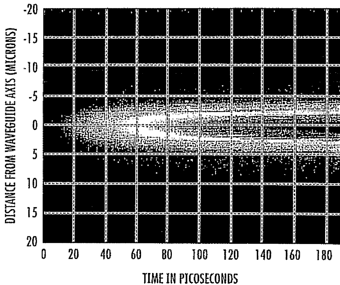
TRANSIENT FIELD PATTERNS IN RESONATOR GUIDE
