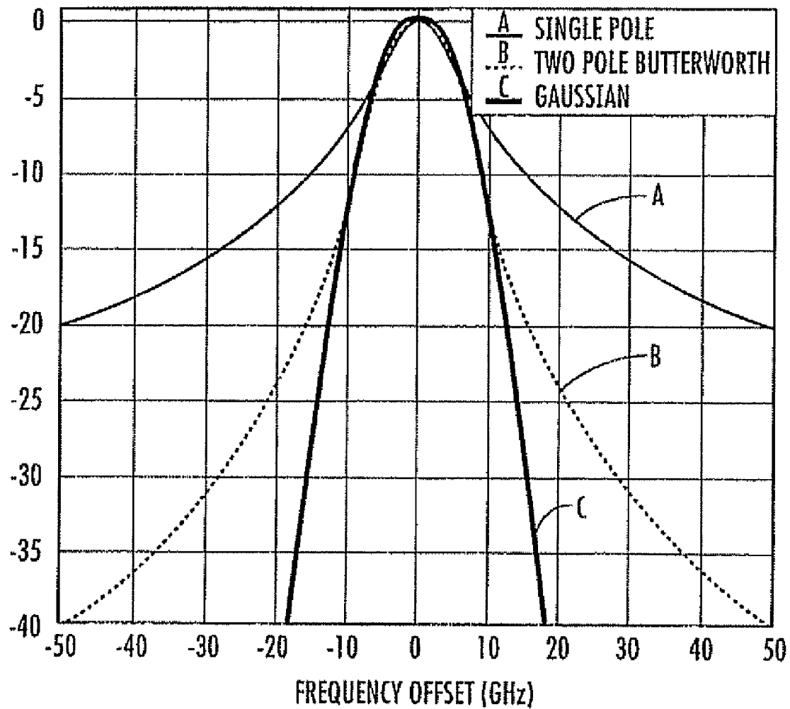
BANDSHAPE FOR GAUSSIAN AND BUTTERWORTH FILTERS
