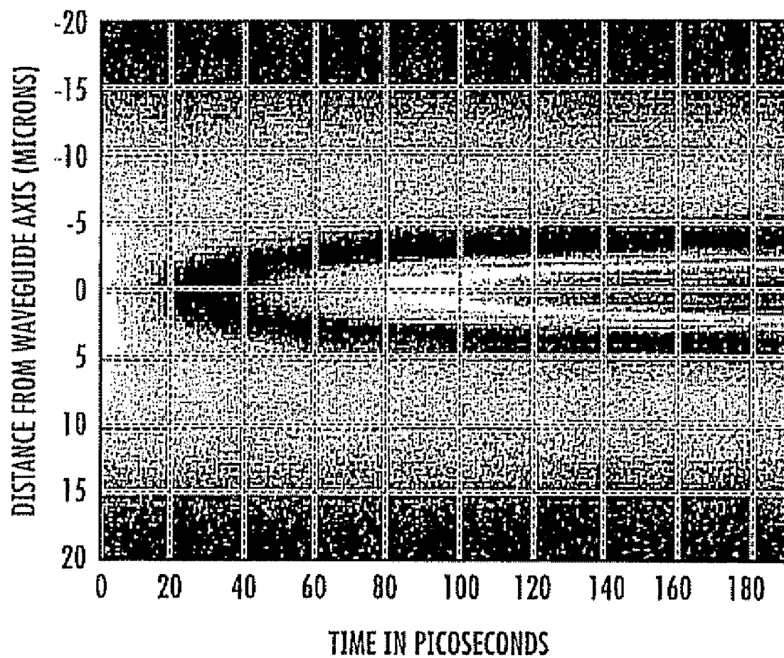
TRANSIENT FIELD PATTERNS IN SOURCE GUIDE
