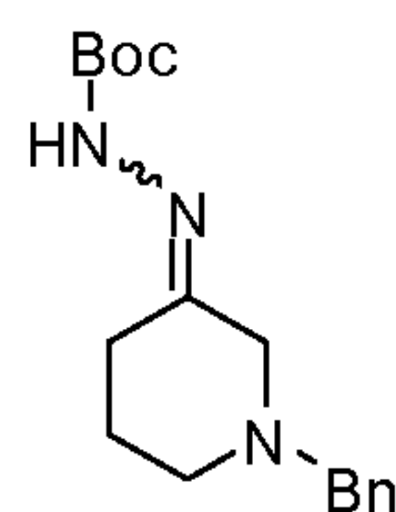
XV-Bn
