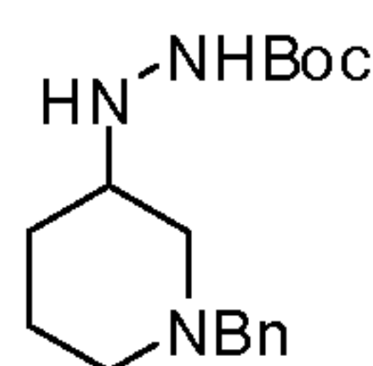
XV-Bn
