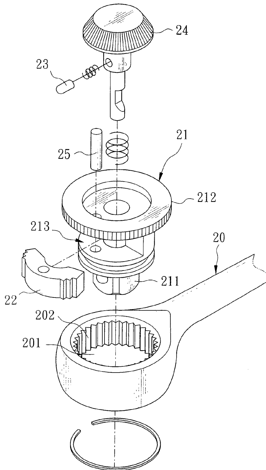
FIG. 3 PRIOR ART
