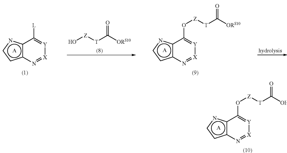
(Reaction Scheme 5)
