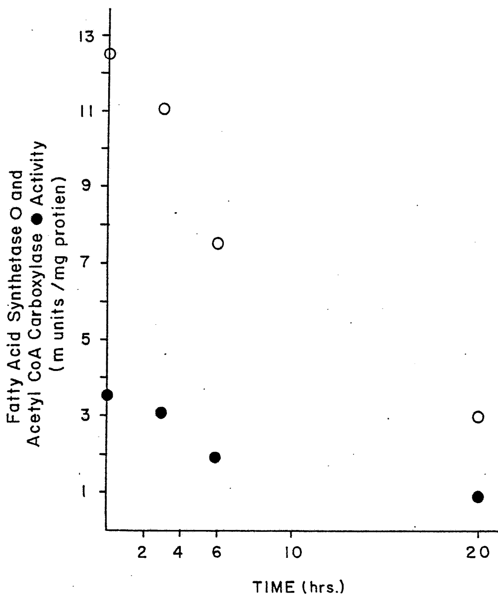
FIG.4: Effect of conditioned medium from endotoxin-treated mouse peritoneal exudate cells on the activities of acetyl CoA carboxylase and fatty acid synthetase in 3T3-L1 cells.
