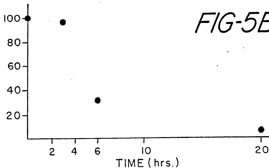
FIG. 5A & 5B: Effect of mediator that suppresses the synthesis of fatty acid synthetase.
