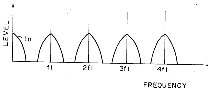
FIG. 4C PRIOR ART
