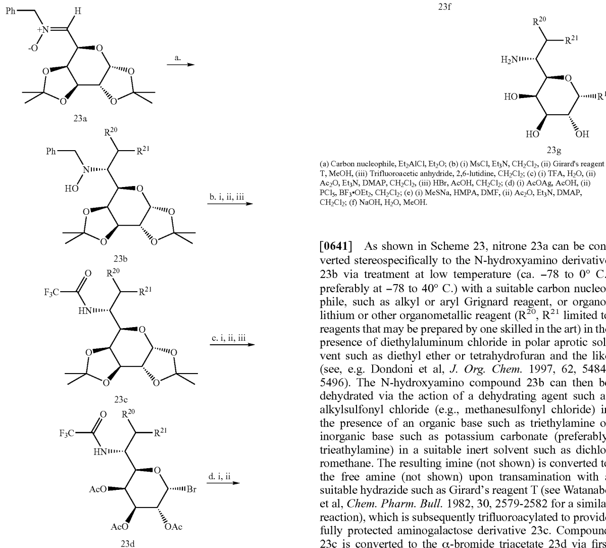
Scheme 23. General synthesis of C6 lincosamine derivatives.
