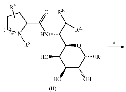
Scheme 28. General synthesis of 2-substituted esters defined for structures of type (II).
