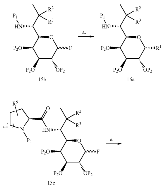
Scheme 16. Displacement of Fluoro by Sulfanyl Moiety
