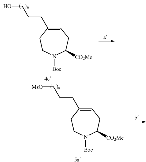
Scheme 5'. Preparation of 5-(hydroxyalkyl)-2,3,6,7-tetrahydroazepine-1,2-dicarboxylic acid 1-tert-butyl ester 2-methyl ester intermediates by nucleophilic displacement.
