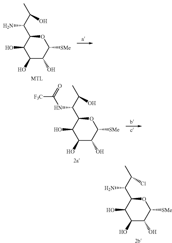
Scheme 2'. Preparation of 7-Chloro MTL (2b').
