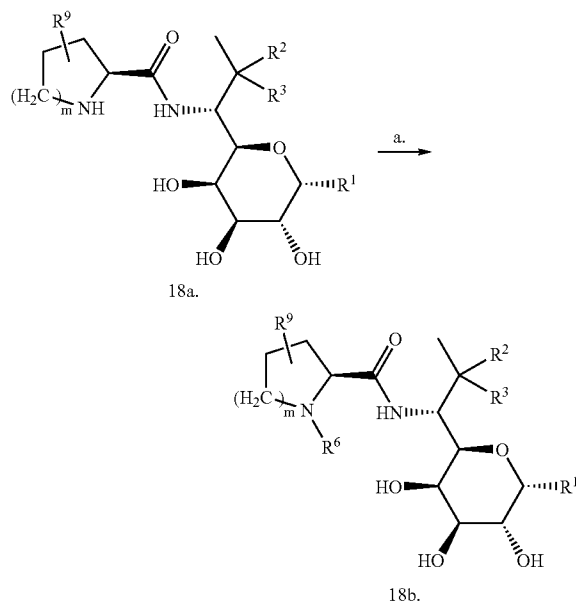
Scheme 19. General synthesis of 1'-N-substituted lincosamides.
