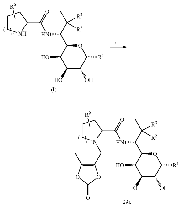
Scheme 29. general synthesis of R 6 dioxalinone prodrugs
