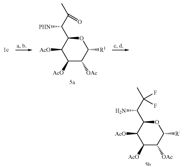
Scheme 5. General synthesis of 7-deoxy-7,7-difluorolincosamines 5b.
