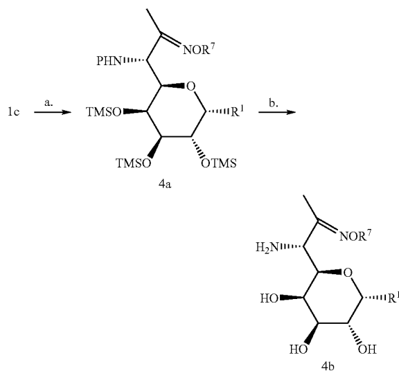
Scheme 4. General synthesis of 7-oxime-lincosamines 4b.
