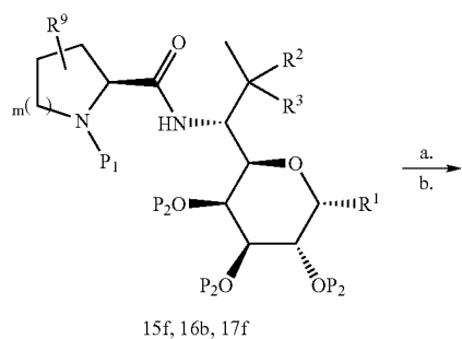
Scheme 18. Global deprotection 15f, 16b, and 17f to compounds of formula (I).
