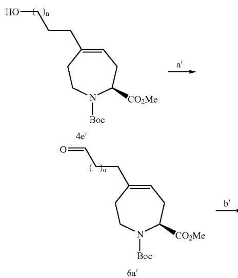
Scheme 6'. Synthesis of 5-(difluoro-alkyl)-2,3,6,7-tetrahydroazepine-1,2-dicarboxylic acid 1-tert-butyl ester 2-methyl ester intermediates 6b'.
