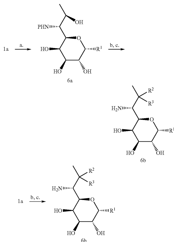
Scheme 6. General synthesis of 7-deoxy-7-halolincosamines 6b.
