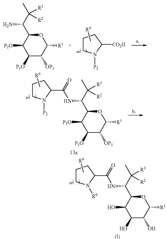
Scheme 13. General coupling and deprotection methods.
