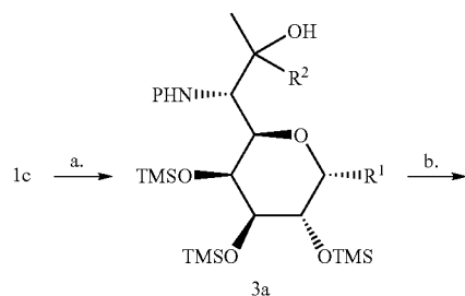
Scheme 3. General synthesis of lincosamine intermediate 3b.
