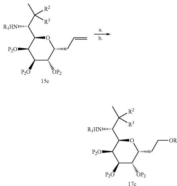
Scheme 17. General synthesis of alcohol and ether 1-position lincosamine derivatives
