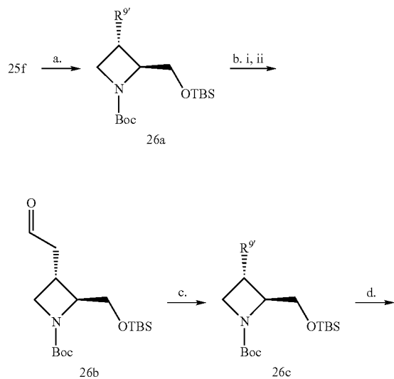
Scheme 26. General synthesis of trans-alkylazetidinecarboxylic acids via aldehyde.
