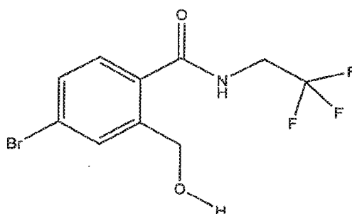
2-(2,2,2-trifluoroethyl)-5-mercaptoisoindolin-1-one
