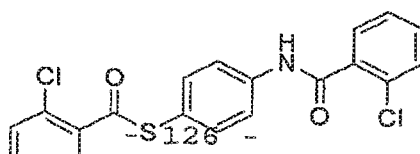
2-chloro-N-(4-mercaptophenyl)benzamide
