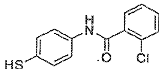
2-chloro-N-(4-mercaptophenyl)benzamide
