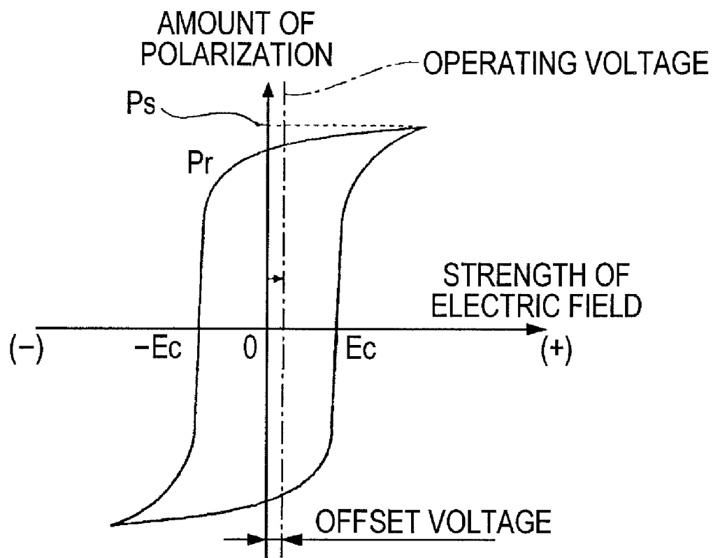
HYSTERESIS LOOP OF PIEZOELECTRIC MATERIAL (P-E CURVE)
