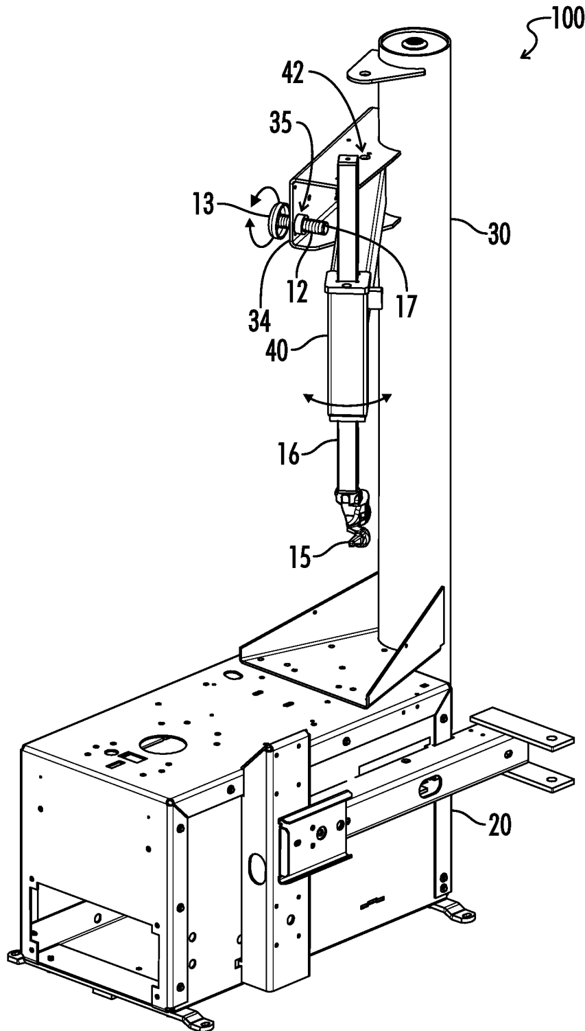
FIG. 1 (PRIOR ART)
