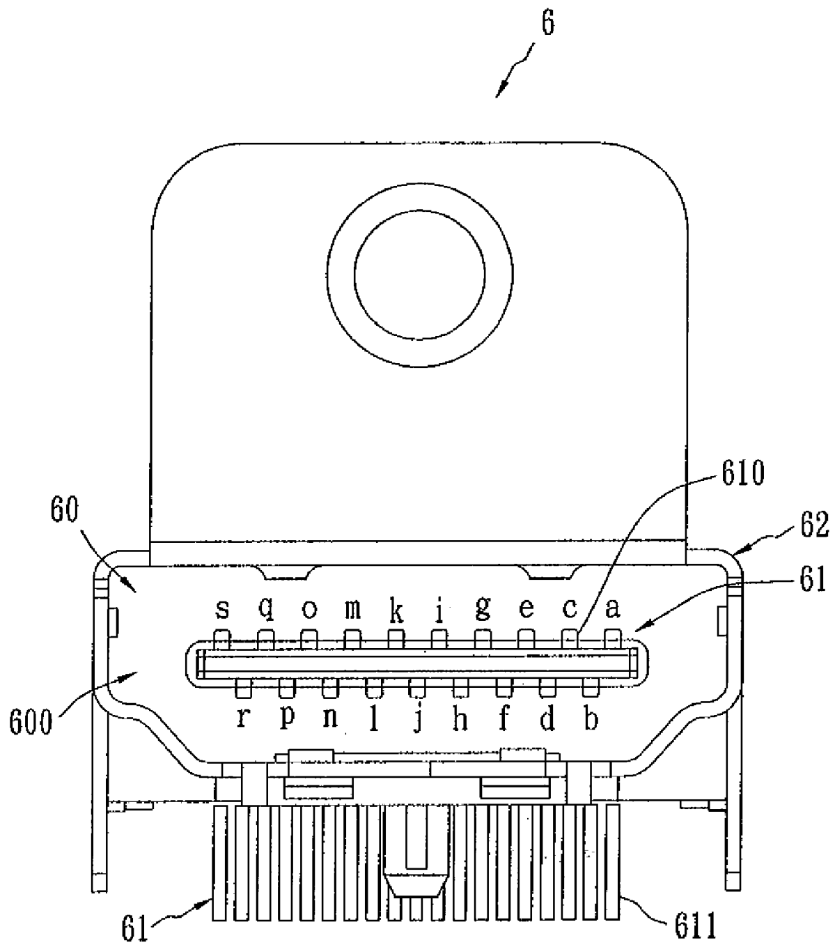
FIG. 1 (Prior Art)
