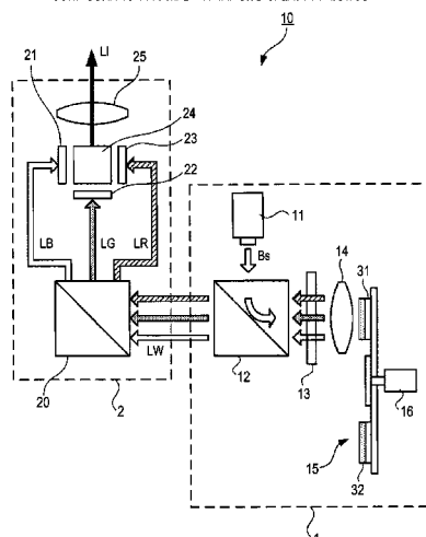
CONFIGURATION EXAMPLE OF IMAGE DISPLAY APPARATUS
