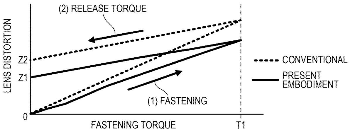
RELATION BETWEEN FASTENING TORQUE AND LENS DISTORTION
