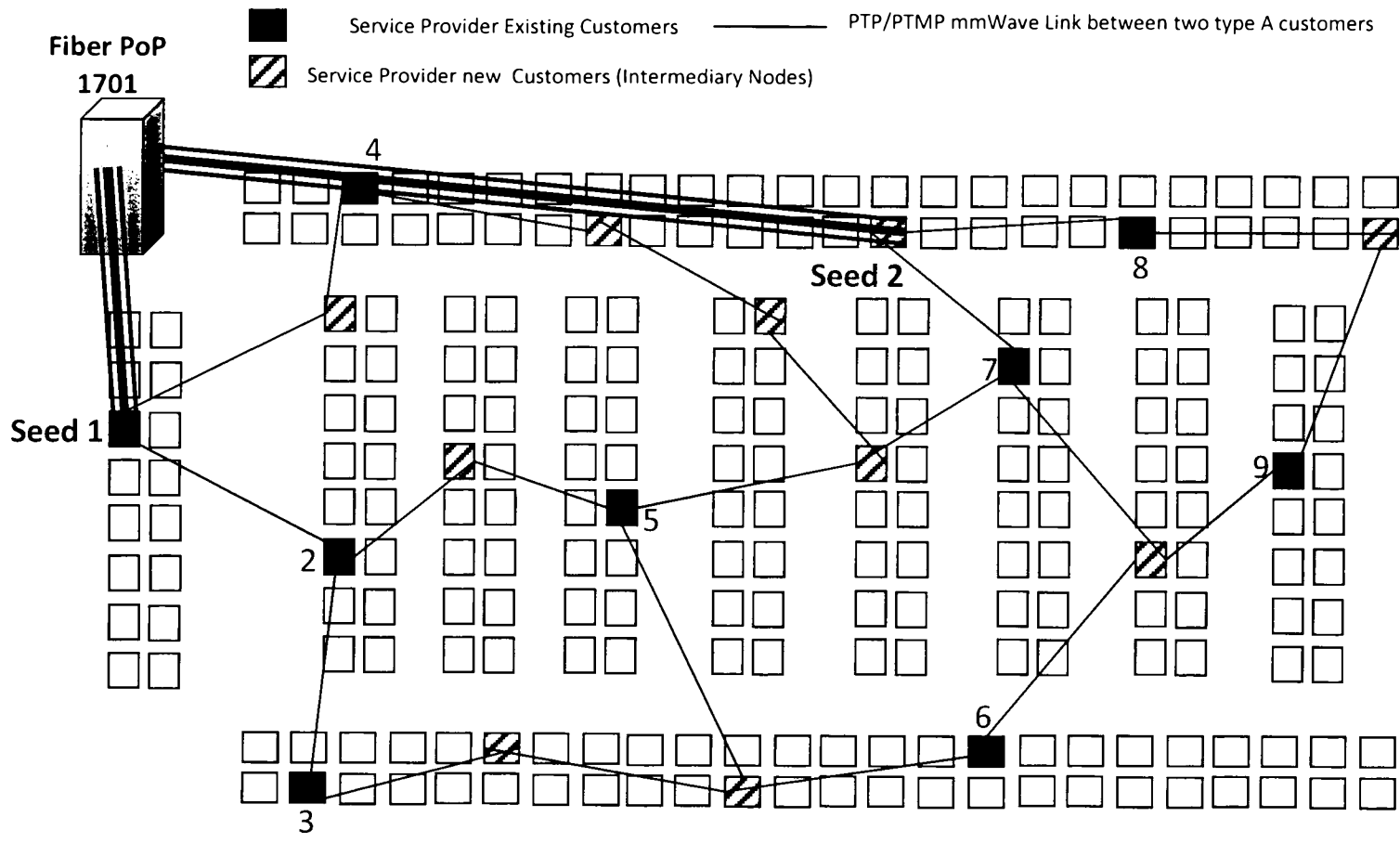
Service Provider Wireless Mesh Communication network 1700
