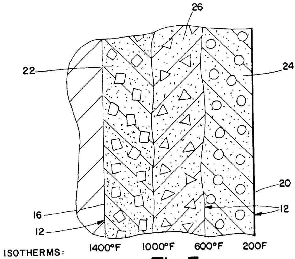
Fig. 3 (PRIOR ART)
