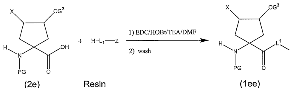
Scheme 6
