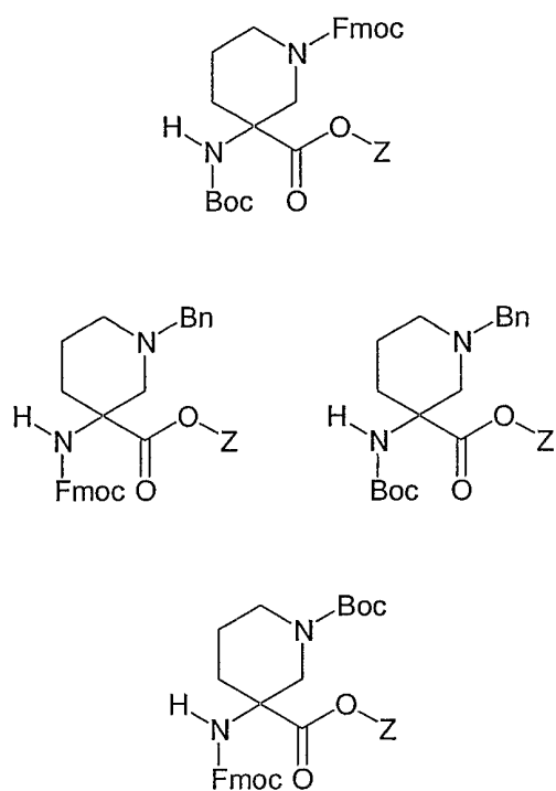
Figure 8 Z = Merrifield resin
