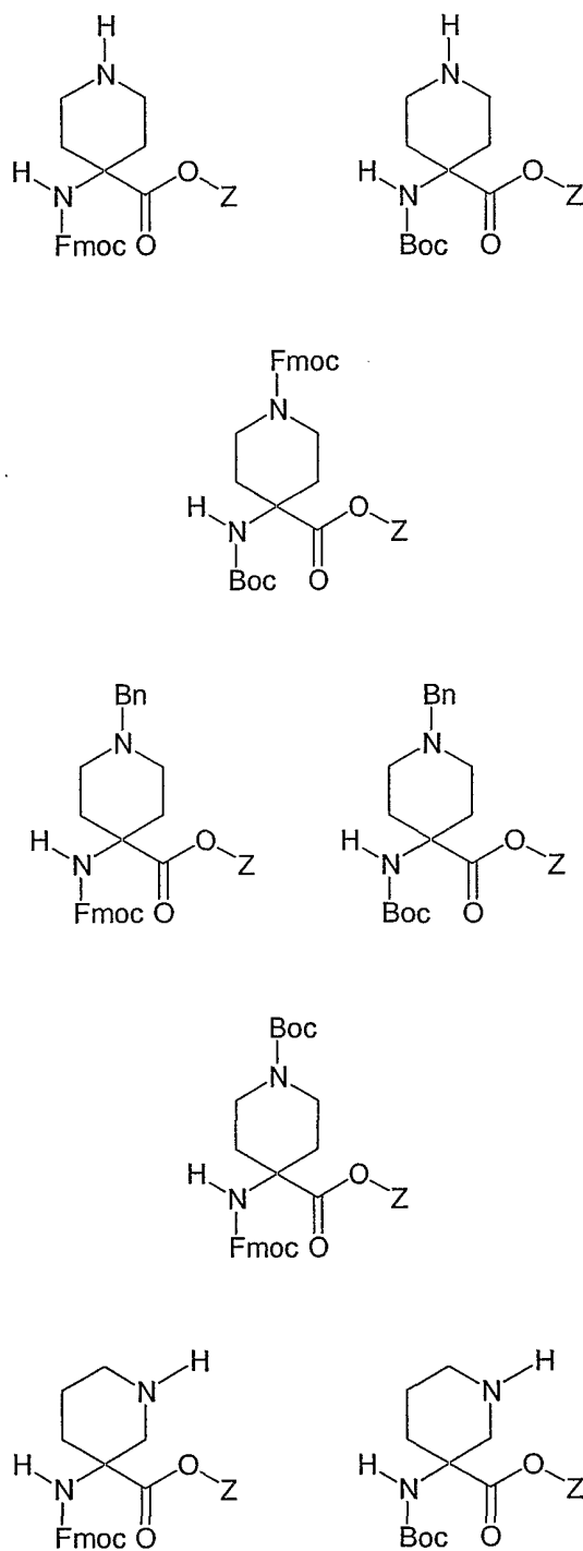
Figure 3 Z = Wang Resin
