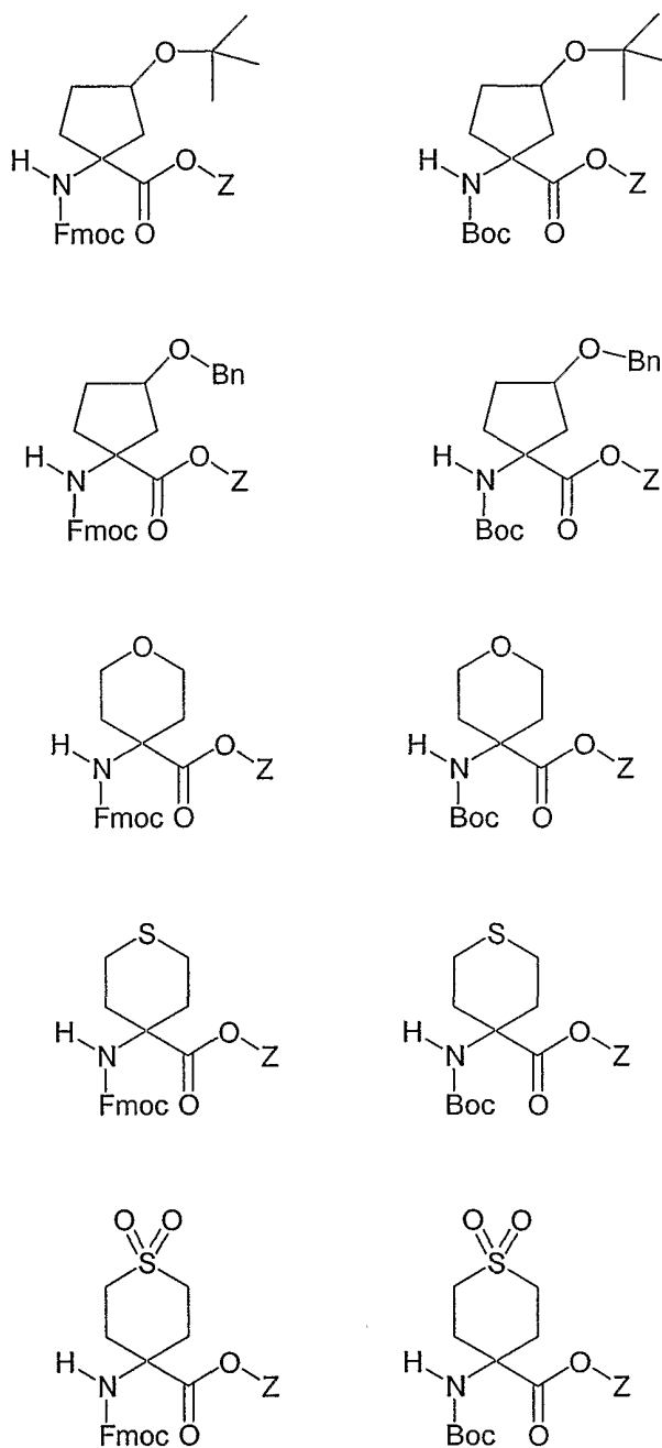
Figure 2 Z = Wang Resin
