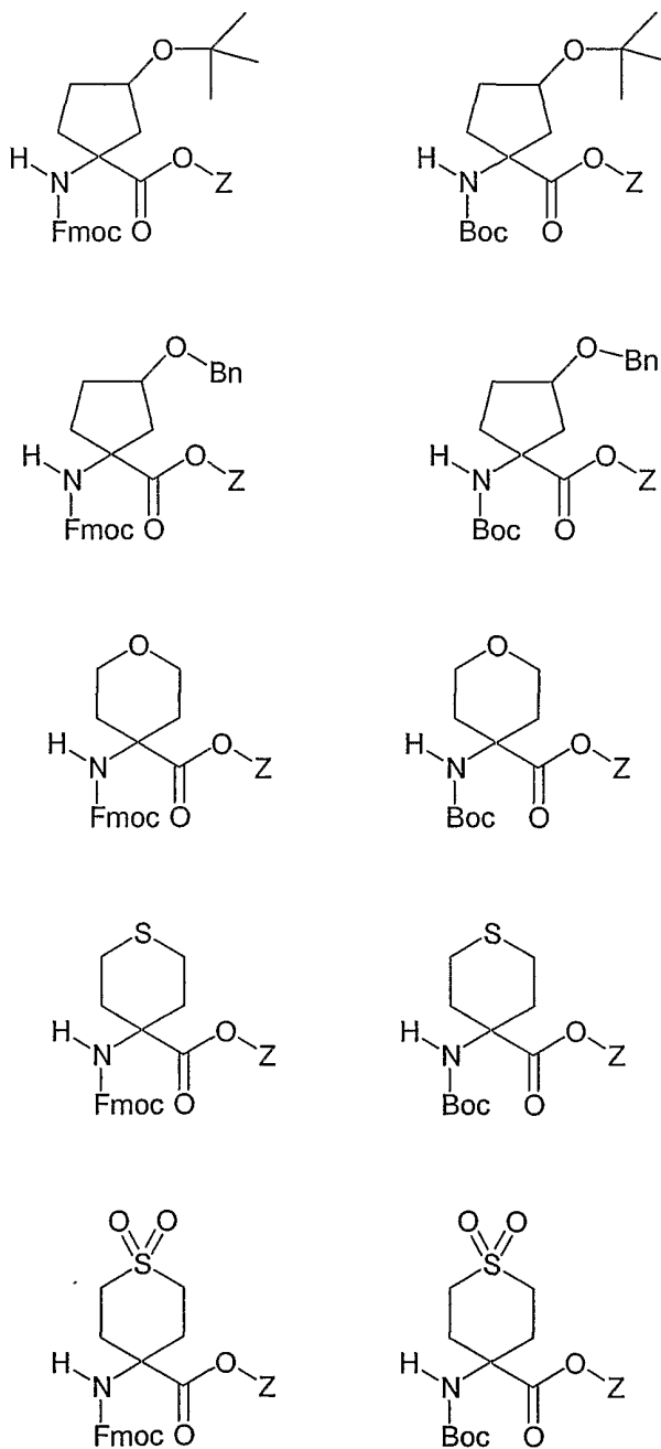
Figure 6 Z = Merrifield resin
