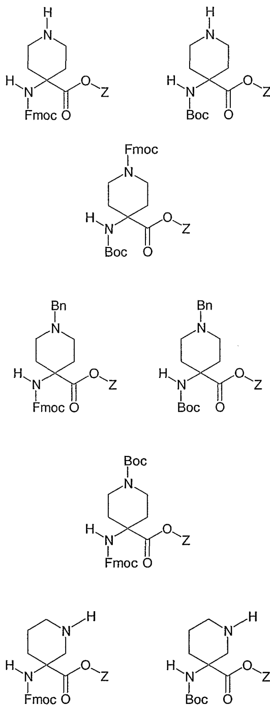
Figure 7 Z = Merrifield resin
