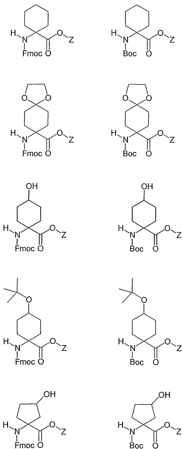
Figure 5 Z = Merrifield resin
