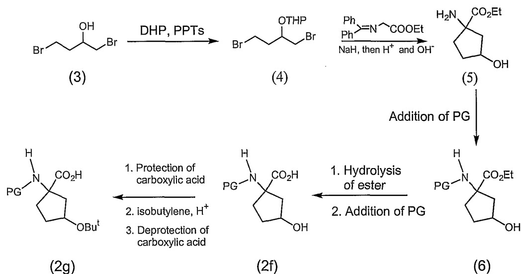
Scheme 9
