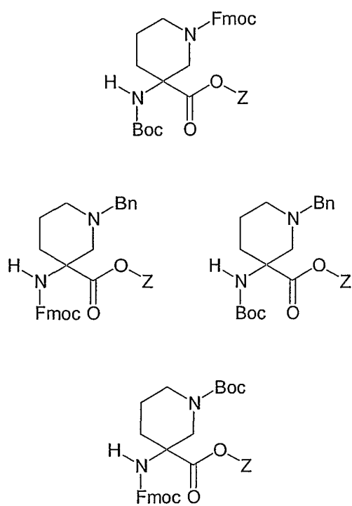
Figure 4 Z = Wang resin
