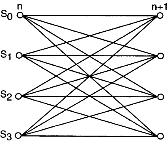
FIG. 2C PRIOR ART
