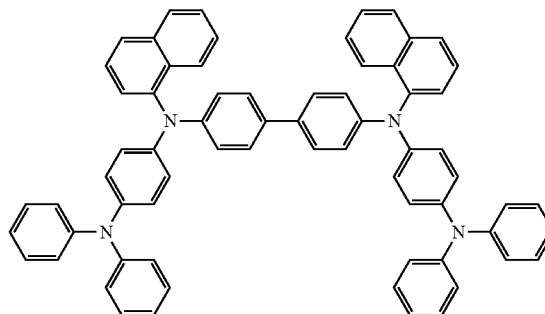
Compound BD2
