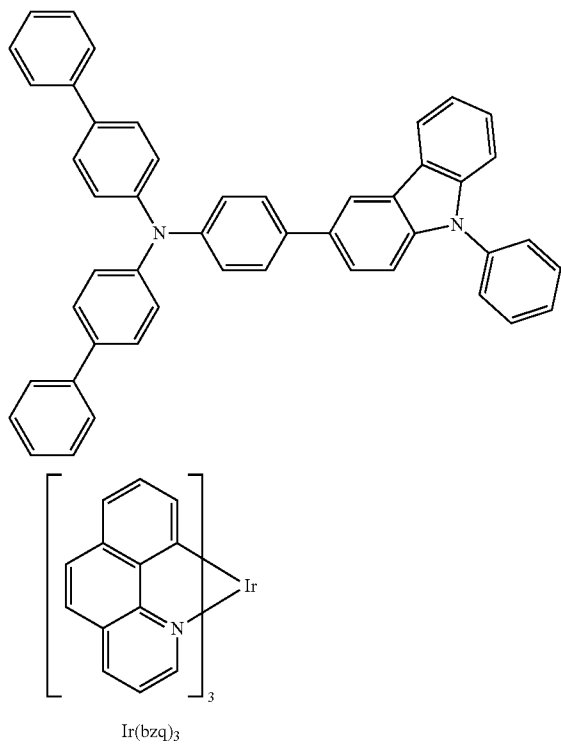
Compound ET
