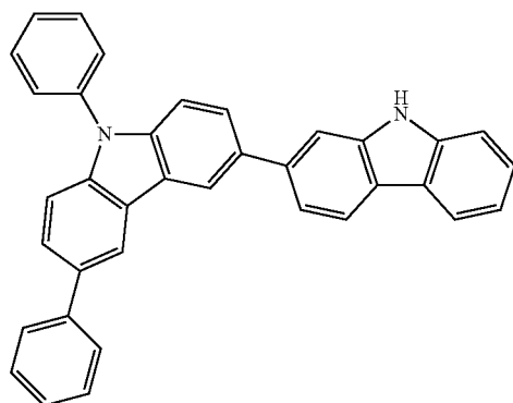
Intermediate 13
