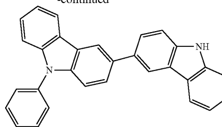
Intermediate 4
