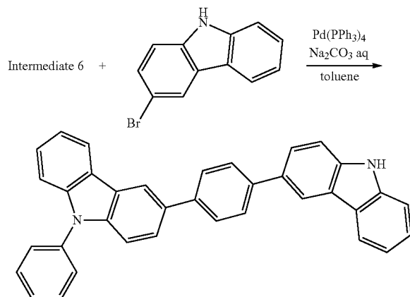
Intermediate 7
