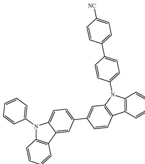
Compound H4
