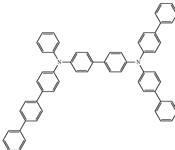
Compound X1
