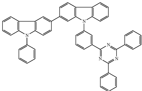
Compound F2
