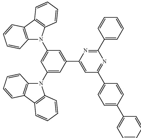
Compound BH1
