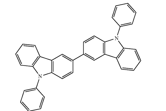
Compound F2
