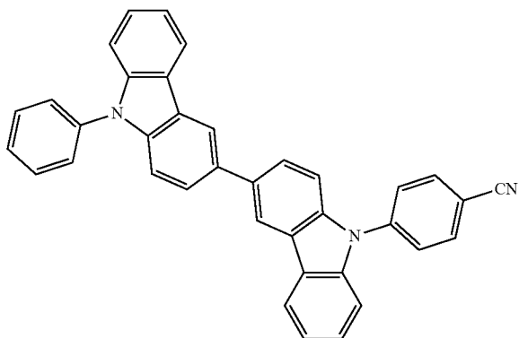
Compound H6
