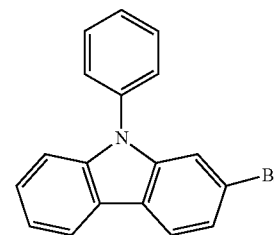
Intermediate 14
