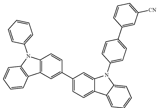
Compound H2
