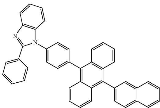
Compound H1
