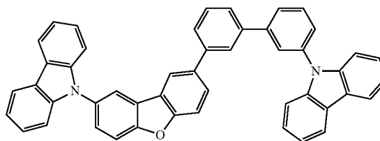
Compound F4
