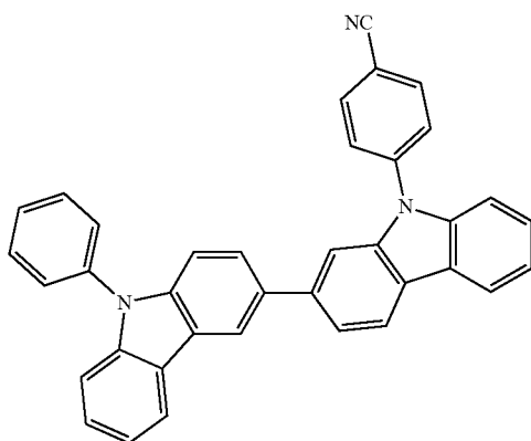
Compound H1
