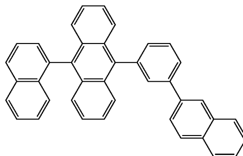
Compound BD1
