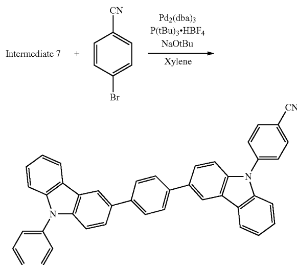
H12
