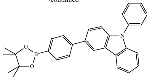
Intermediate 6
