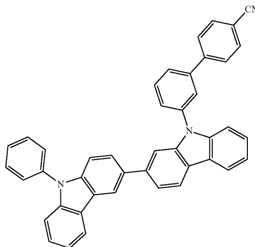
Compound H4
