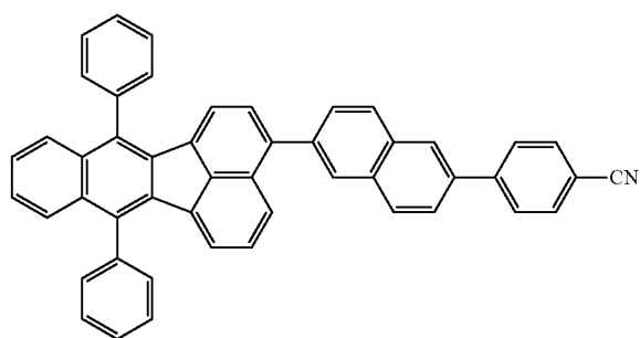
Compound BD1
