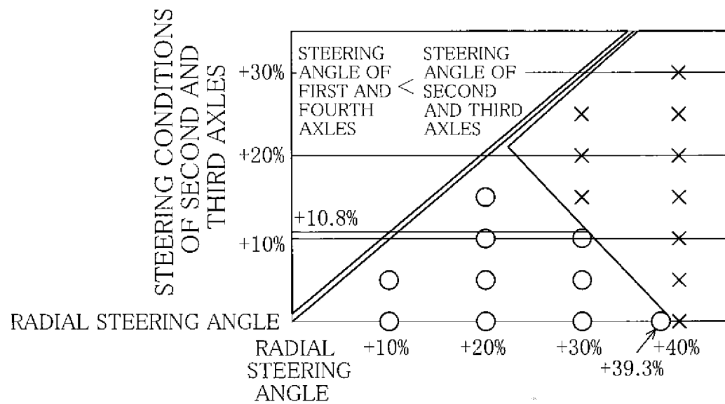
STEERING CONDITIONS OF FIRST AND FOURTH AXLES
