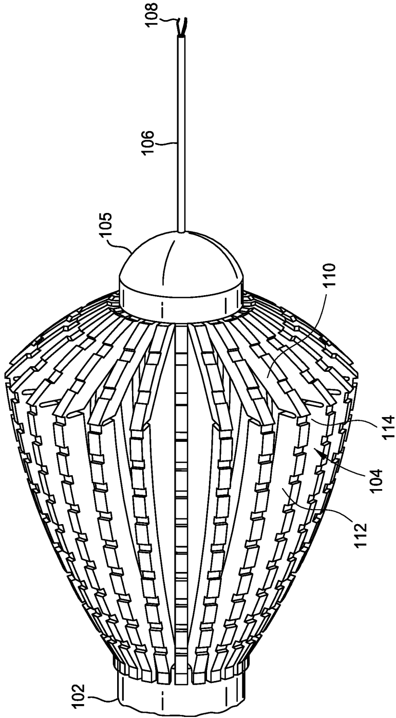
Fig. 1 (PRIOR ART)
