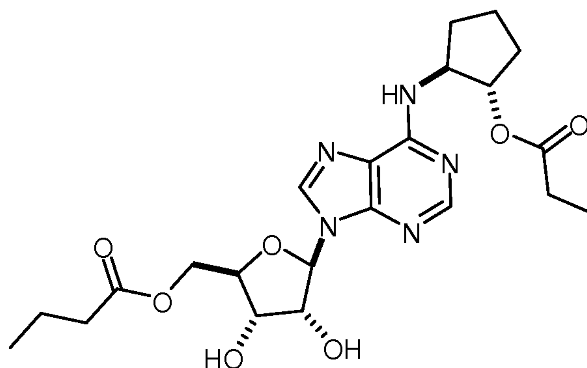
10 ((2R,3S,4R,5R)-5-(6-((1S,2S)-2-(Butyryloxy)cyclopentylamino)-9H-purin-9-yl)-3,4-dihydroxytetrahydrofuran-2-yl)methyl butyrate (3f): MS (ES + ): m/z 392.2 (M+1)
