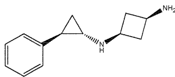
Example 86: (trans)-N1-((1R,2S)-2-phenylcyclopropyl)cyclobutane-1,3-diamine
