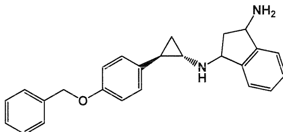
10 Example 71: N1-((trans)-2-(4-(benzyloxy)phenyl)cyclopropyl)-2,3-dihydro-1H-indene-1,3-diamine
