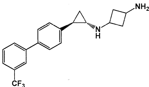
5 Example 69: N1-((trans)-2-(4-(benzyloxy)phenyl)cyclopropyl)cyclobutane-1,3-diamine
