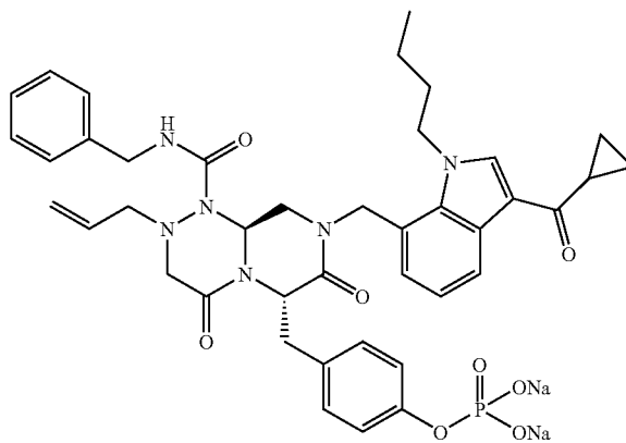
Compound C3
