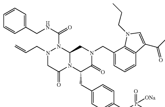
Compound A
