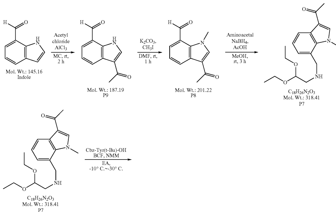
Reaction Scheme 1
