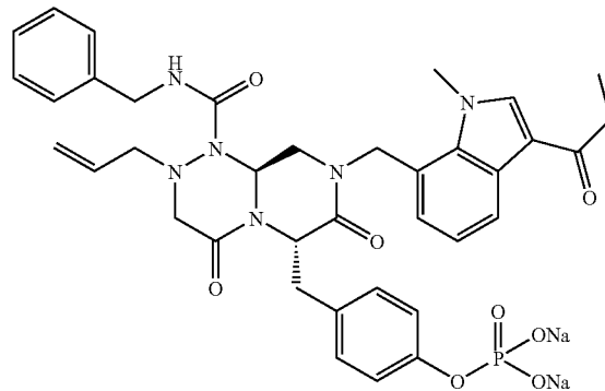
Compound A2
