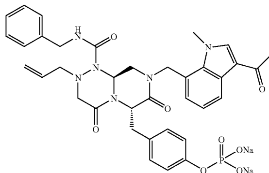
Compound A3
