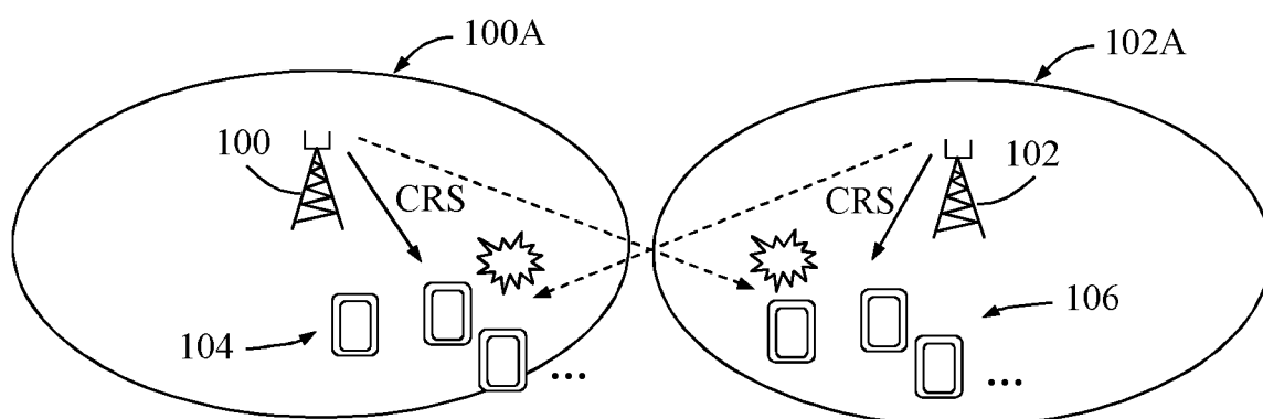
Fig. 2 (prior art)
