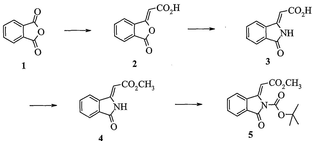
Scheme P1
