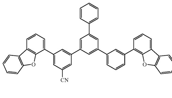
Compound 1A-14
