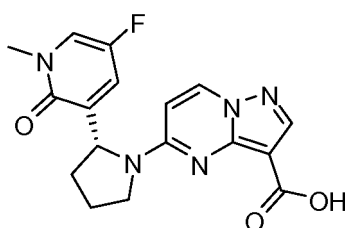
(R)-5-(2-(5-fluoro-1-methyl-2-oxo-1,2-dihydropyridin-3-yl)pyrrolidin-1-yl)pyrazolo[1,5-a]pyrimidine-3-carboxylic acid
