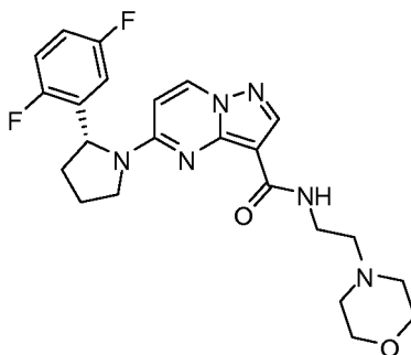
(R)-5-(2-(2,5-difluorophenyl)pyrrolidin-1-yl)-N-(2-morpholinoethyl)pyrazolo[1,5-a]pyrimidine-3-carboxamide
