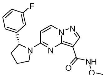
((R)-5-(2-(3-fluorophenyl)pyrrolidin-1-yl)-N-methoxypyrazolo[1,5-a]pyrimidine-3-carboxamide
