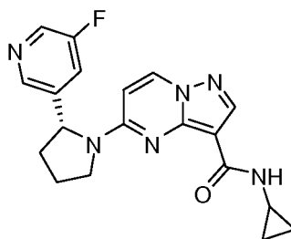
(R)-N-cyclopropyl-5-(2-(5-fluoropyridin-3-yl)pyrrolidin-1-yl)pyrazolo[1,5-a]pyrimidine-3-carboxamide
