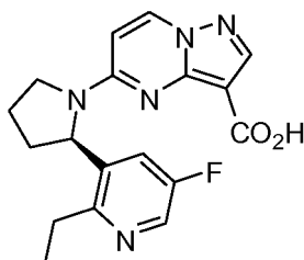
(R)-5-(2-(2-ethyl-5-fluoropyridin-3-yl)pyrrolidin-1-yl)pyrazolo[1,5-a]pyrimidine-3-carboxylic acid
