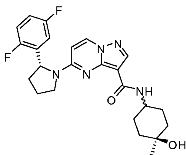
5-((R)-2-(2,5-difluorophenyl)pyrrolidin-1-yl)-N-(4-hydroxy-4-methylcyclohexyl)pyrazolo[1,5-a]pyrimidine-3-carboxamide (Diastereomer 2)
