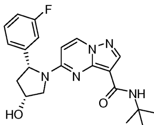
N-tert-butyl-5-((2R,4R)-2-(3-fluorophenyl)-4-hydroxypyrrolidin-1-yl)pyrazolo[1,5-a]pyrimidine-3-carboxamide
