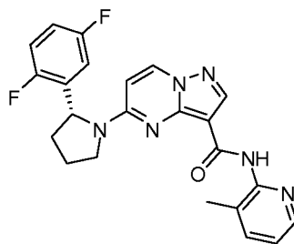
(R)-5-(2-(2,5-difluorophenyl)pyrrolidin-1-yl)-N-(3-methylpyridin-2-yl)pyrazolo[1,5-a]pyrimidine-3-carboxamide
