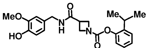
[Chemical Formula 20]
