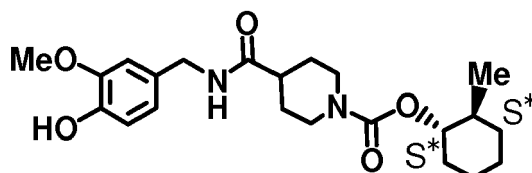
[Chemical Formula 22]
