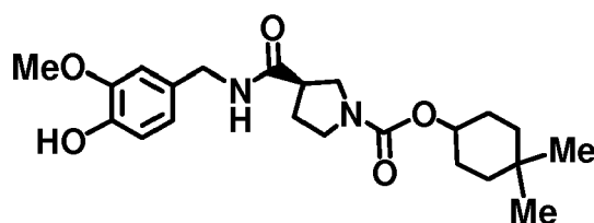
[Chemical Formula 14]
