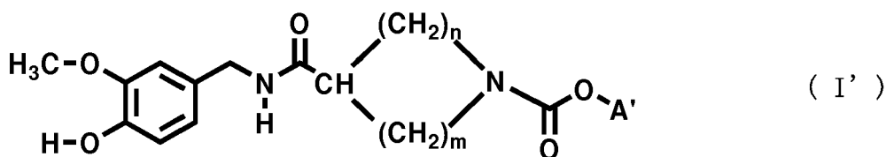
[Chemical Formula 2]
