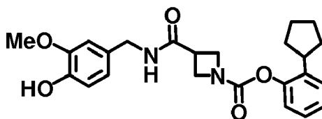
[Chemical Formula 21]
