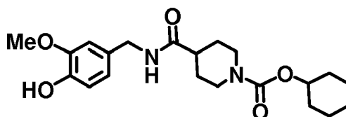
[Chemical Formula 23]
