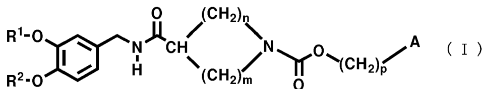
[Chemical Formula 1]
