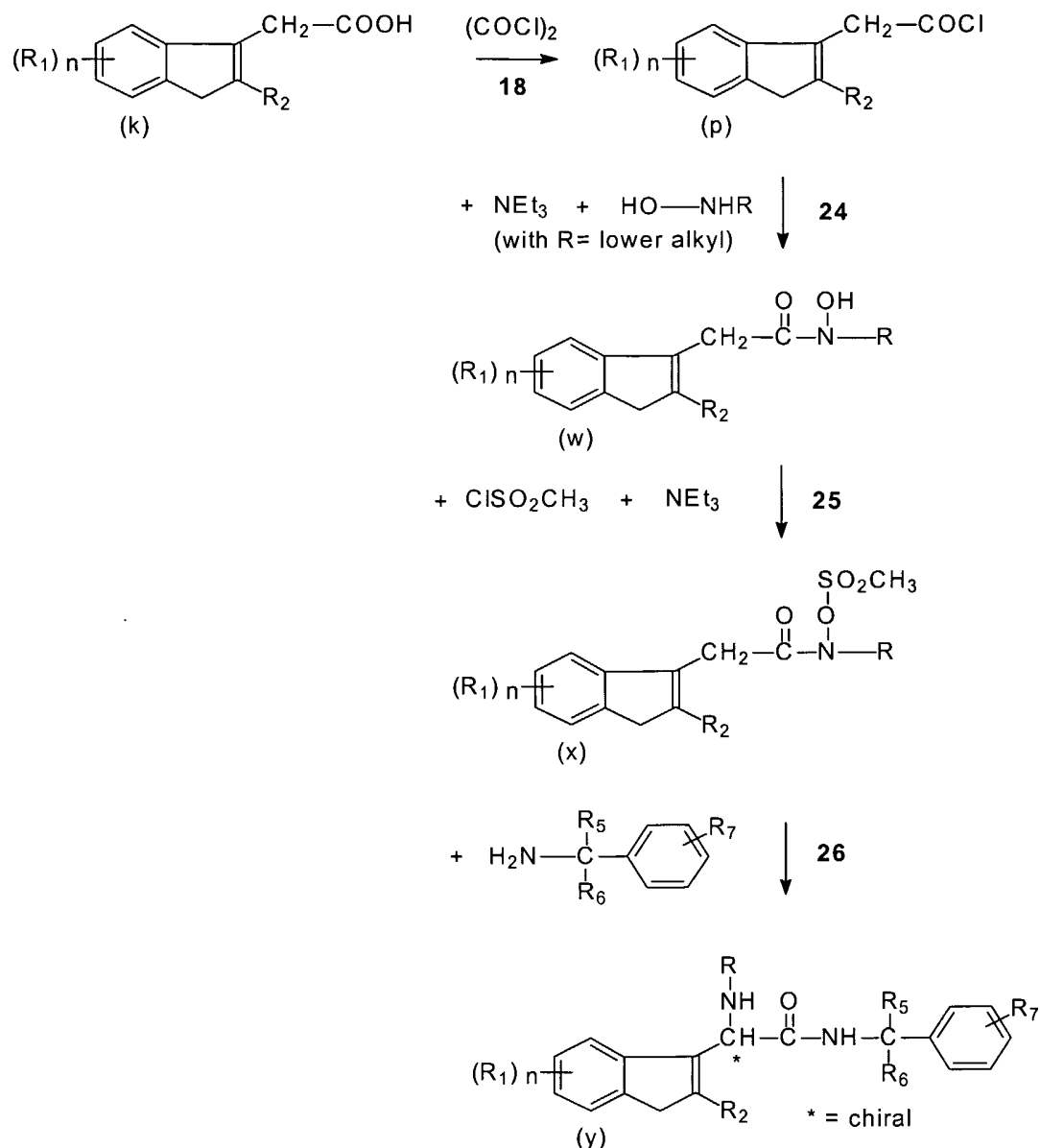
Scheme IIB
