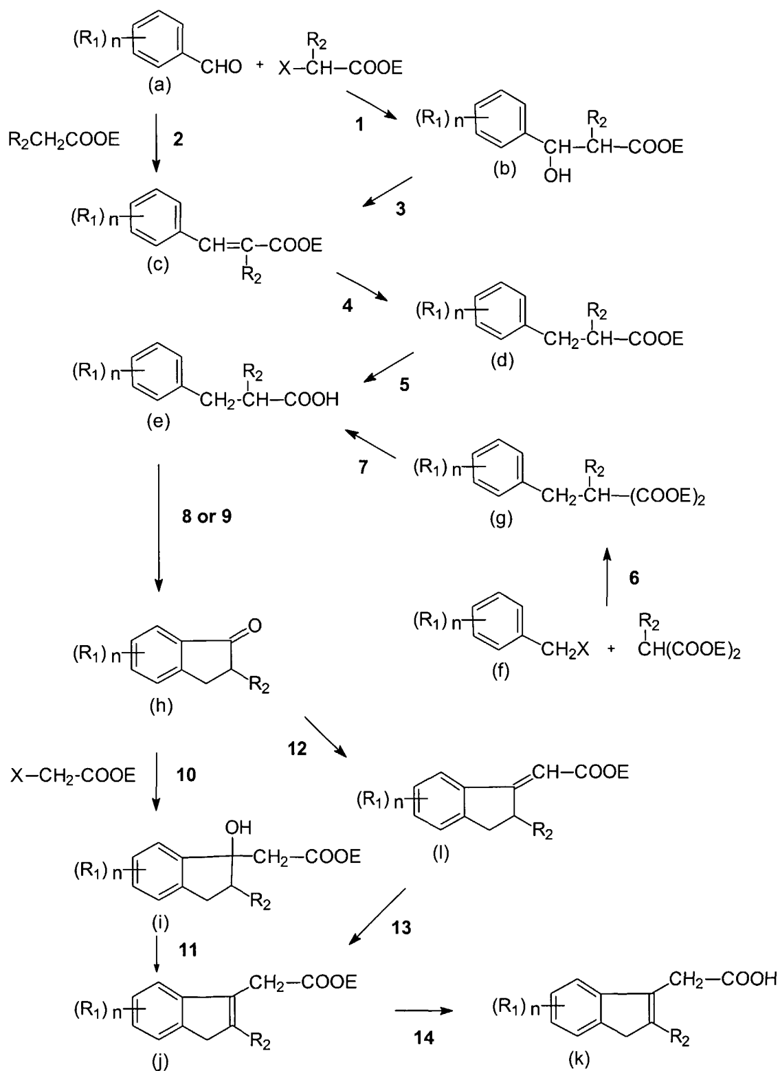
Scheme I
