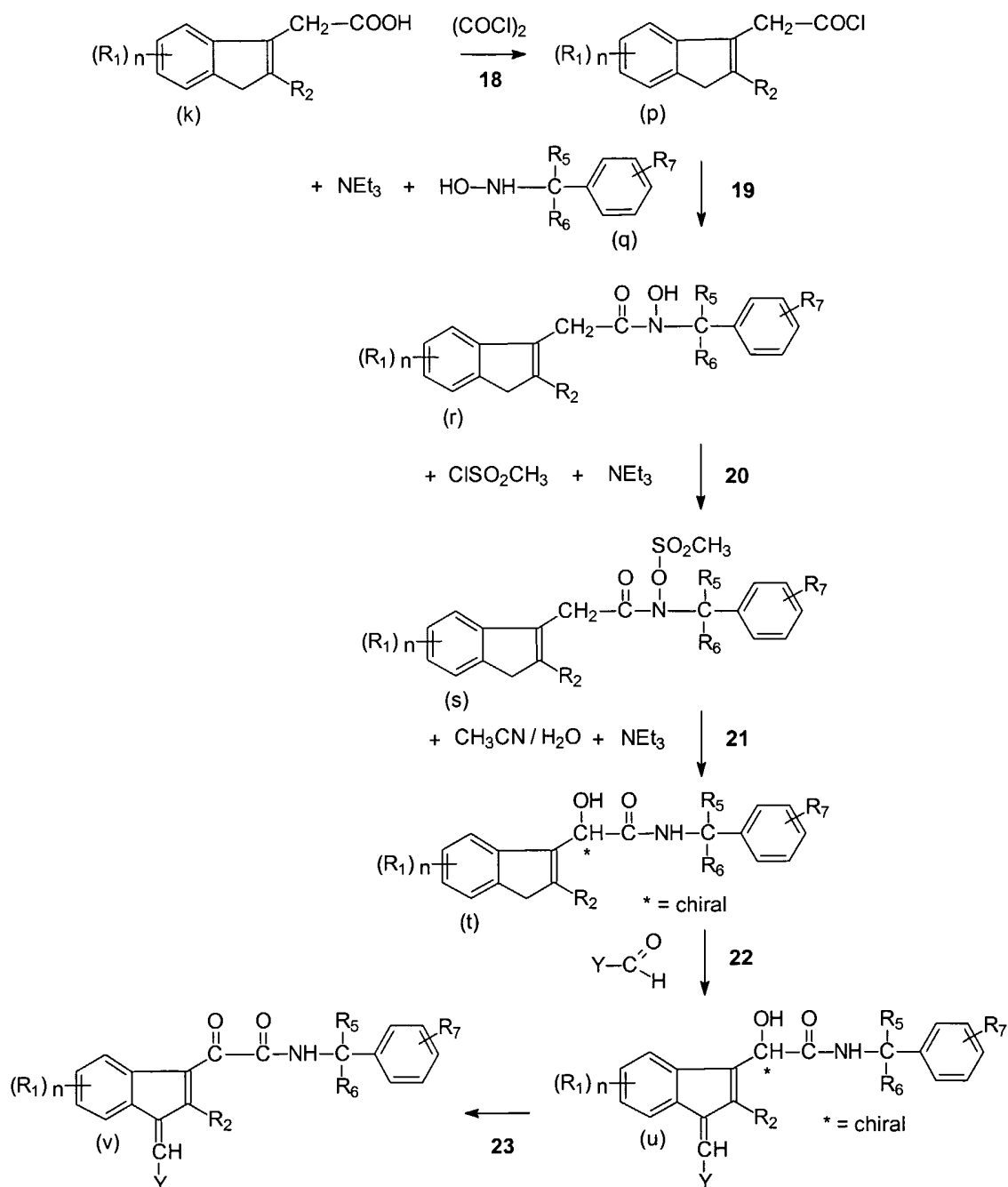
Scheme IIA
