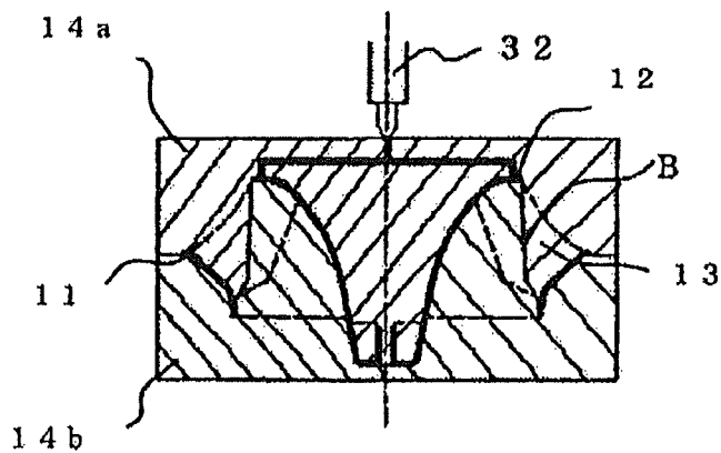
(c) RESIN COOLING STAGE
