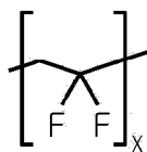
[Chemical Formula 2]
