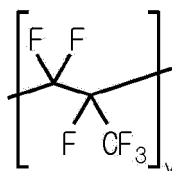
[Chemical Formula 2]
