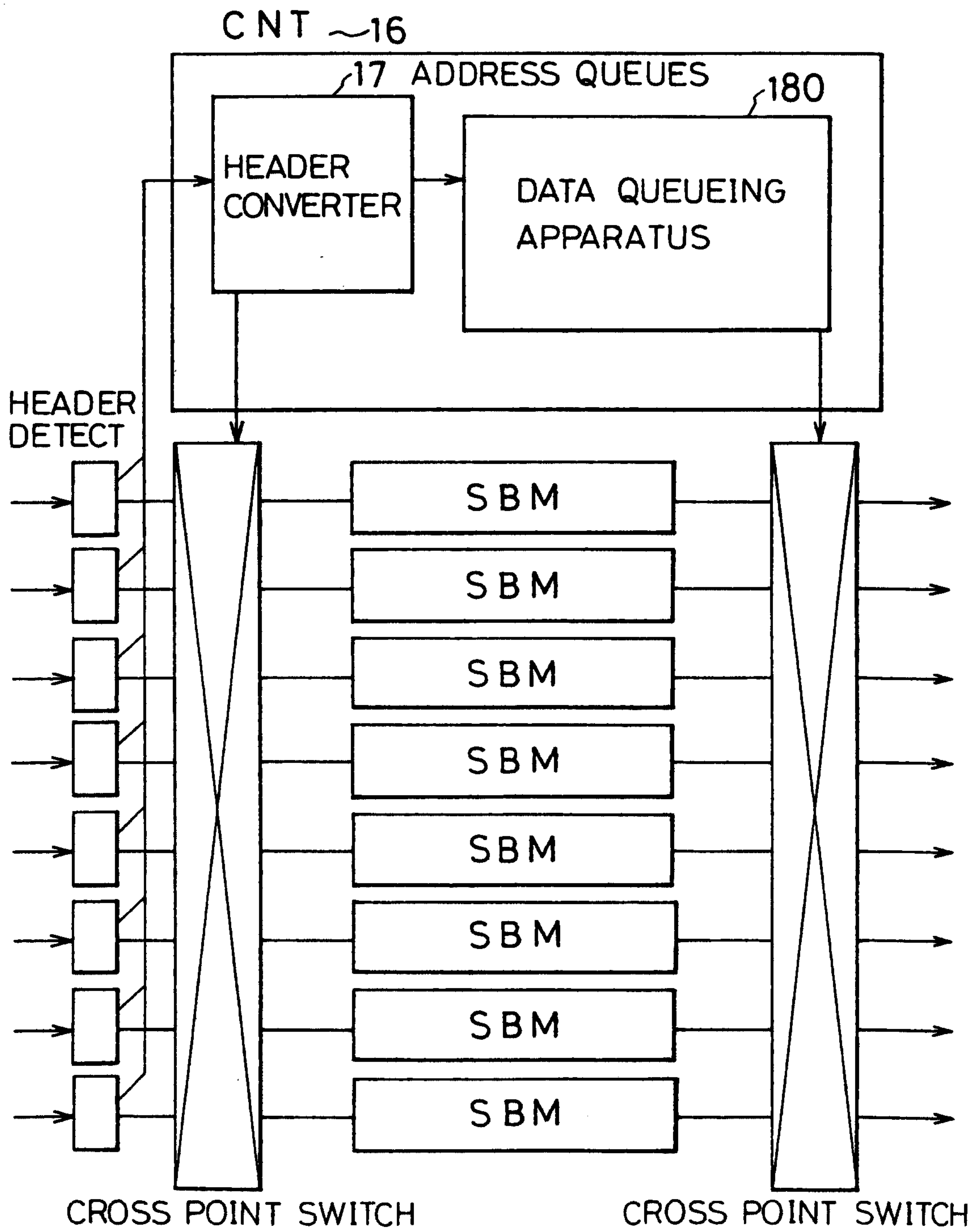
BASIC CONFIGURATION OF SHARED MULTIBUFFER ATM SWITCH
