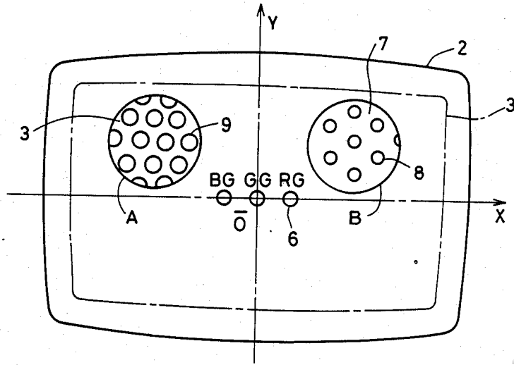
FIG.2 PRIOR ART
