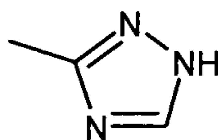
2H-tautomer
