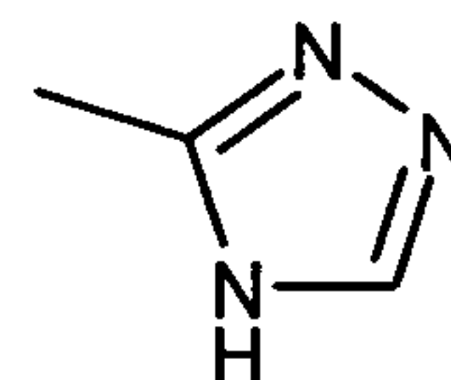
4H-tautomer.
