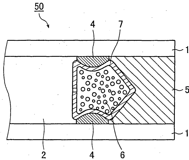
FIG. 5 PRIOR ART
