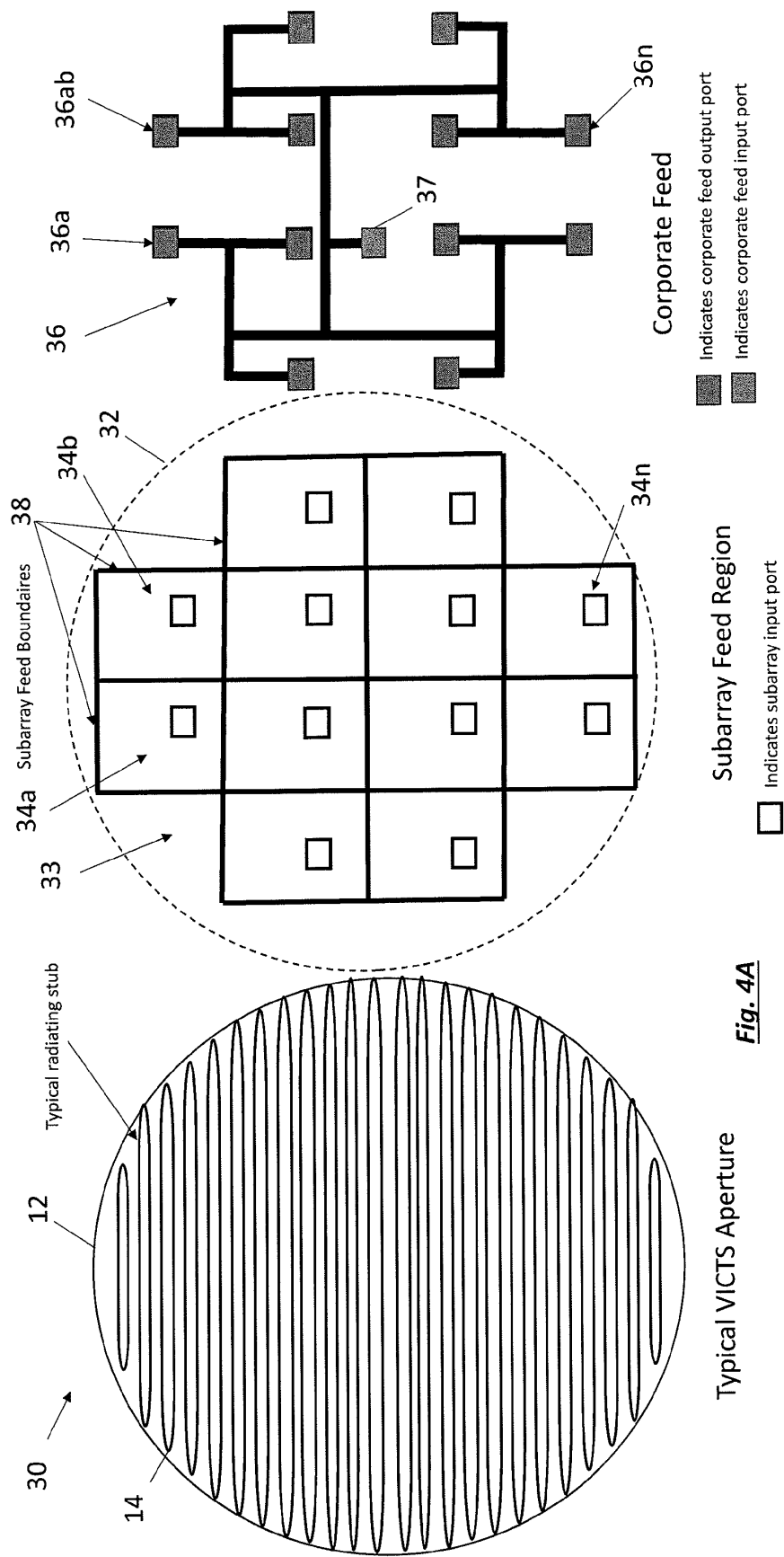
VICTS Array Employing Beam-Stabilization Invention (in both X and Y dimensions)
