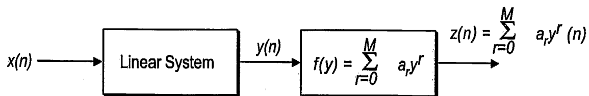
Wiener Model
