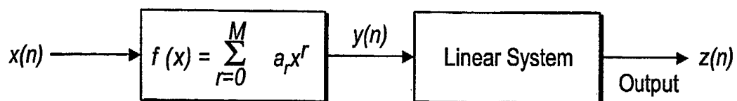
Hammerstein System
