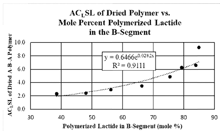
FIG. 3 – Average Chain Sequence Length of Lactoyl Units (ACLSL) of the A-B-A Polymers of Examples 5-12 vs. Mole Percent Polymerized Lactide in the B-Segment
