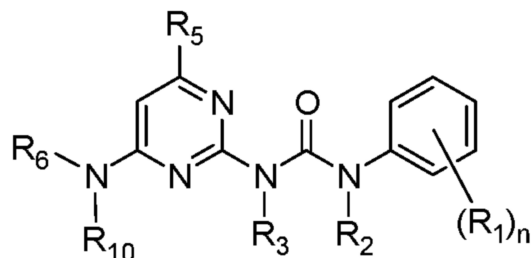
Formula (II);
