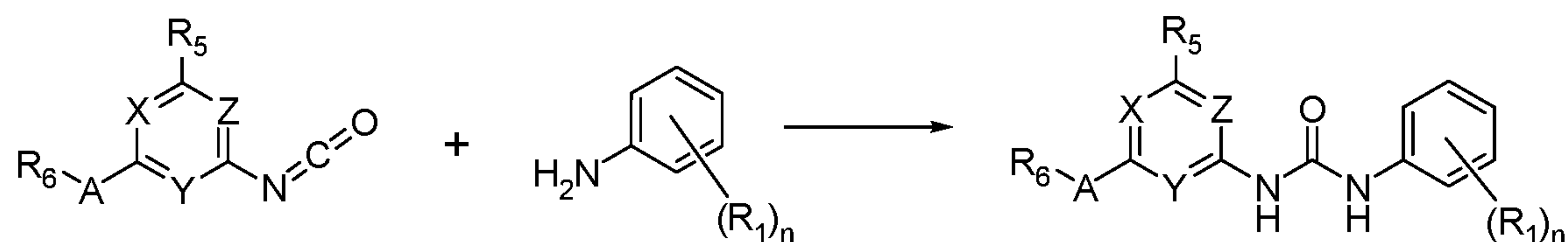
Scheme 1
