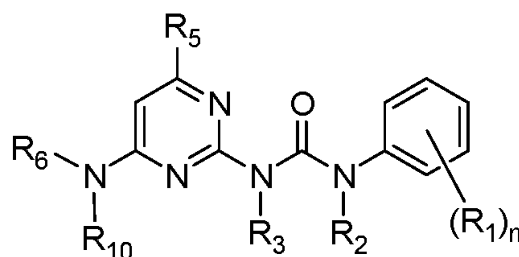
Formula (II);
