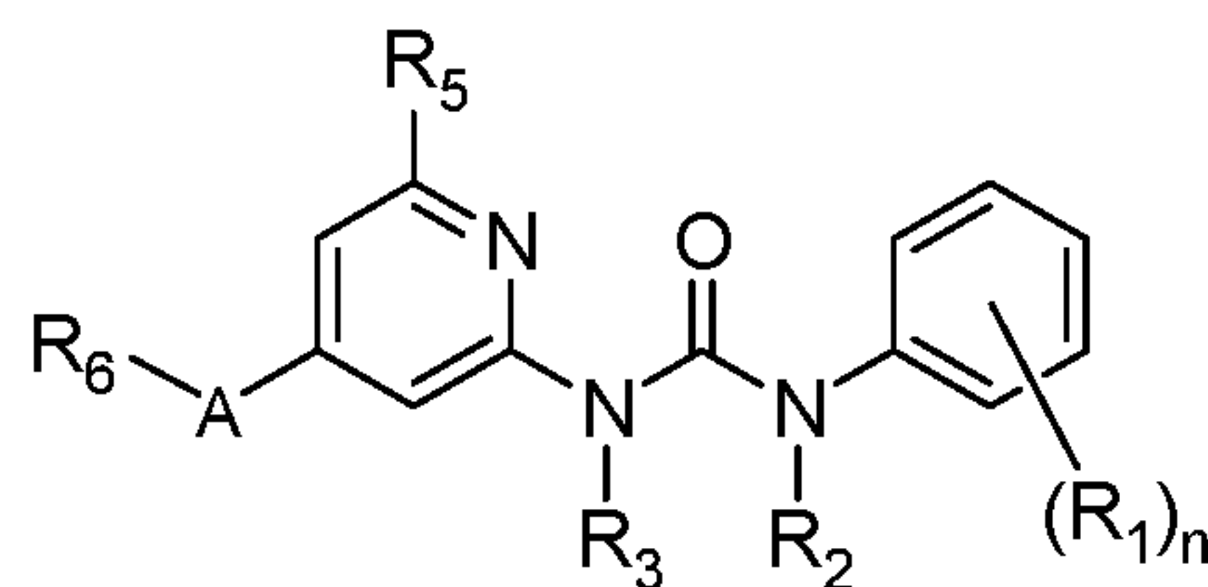
Formula (IV);
