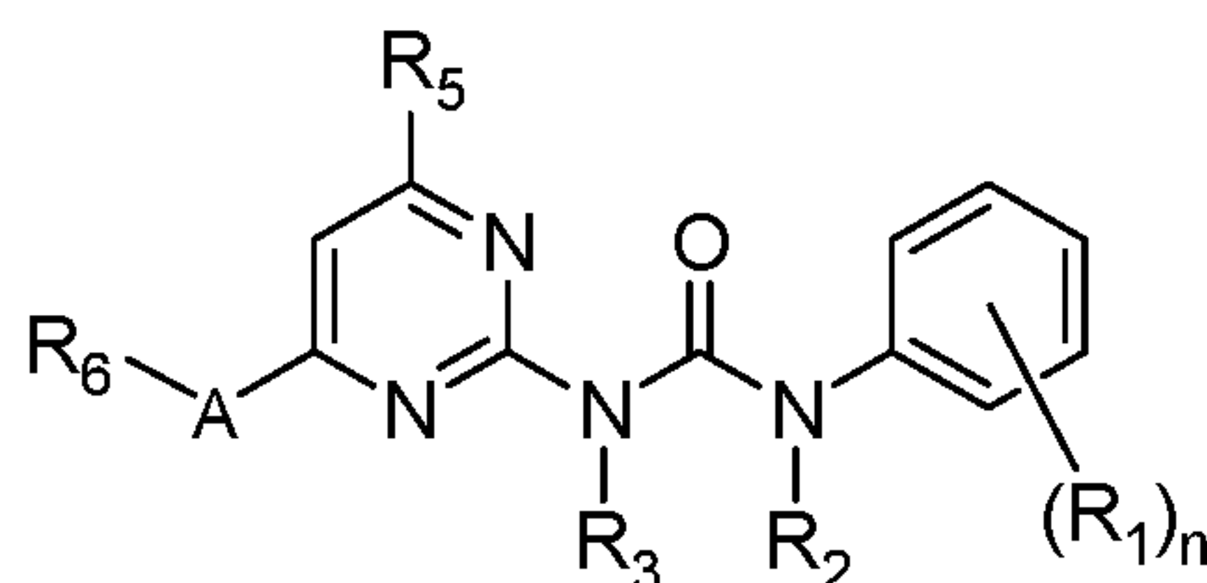
Formula (IIB);
