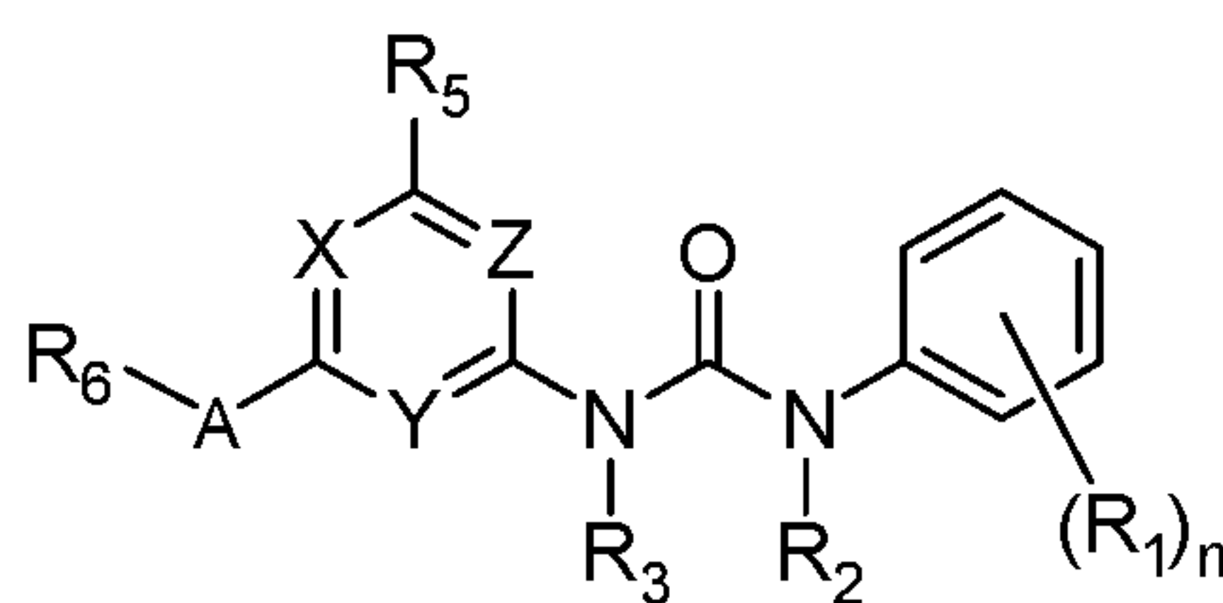
Formula (I);
