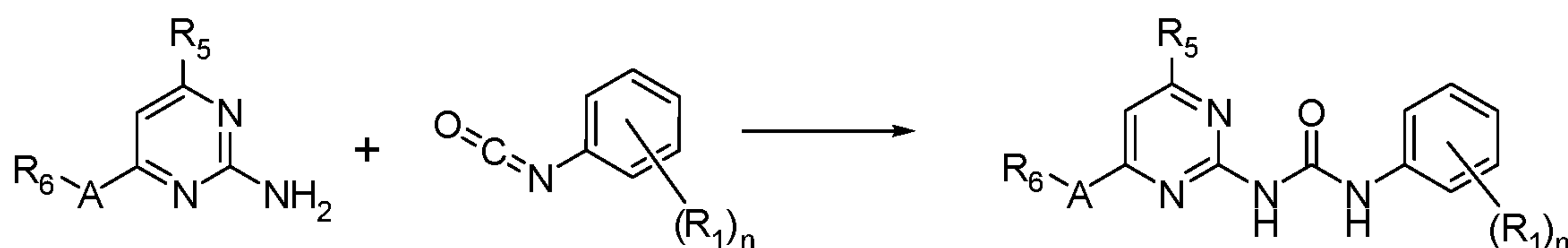
Scheme 2
