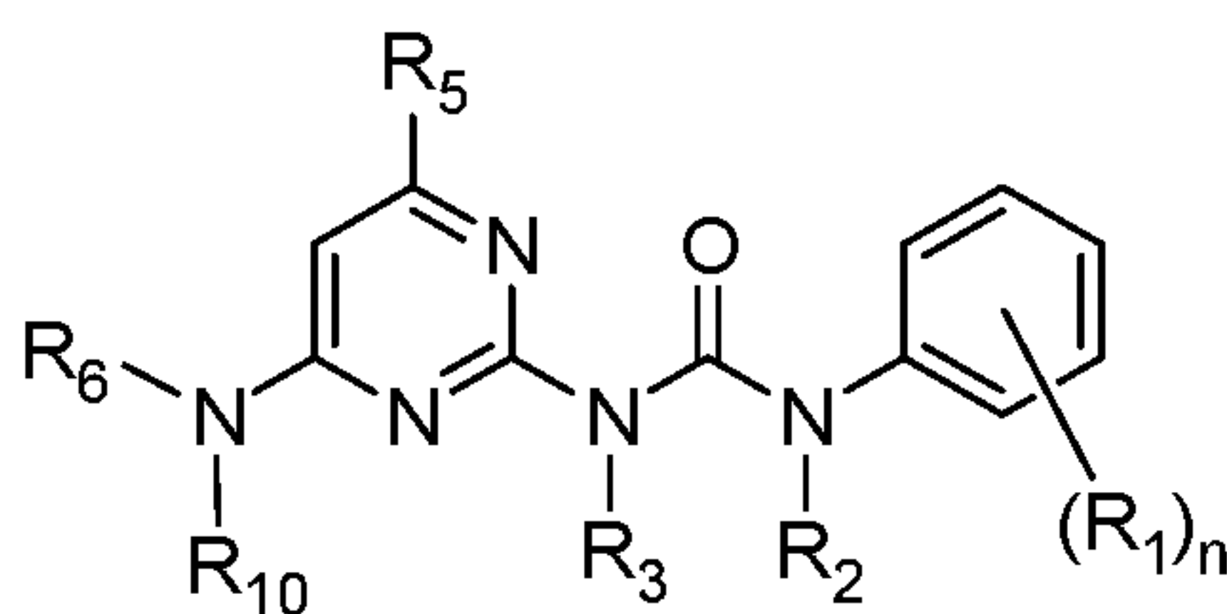
Formula (II);
