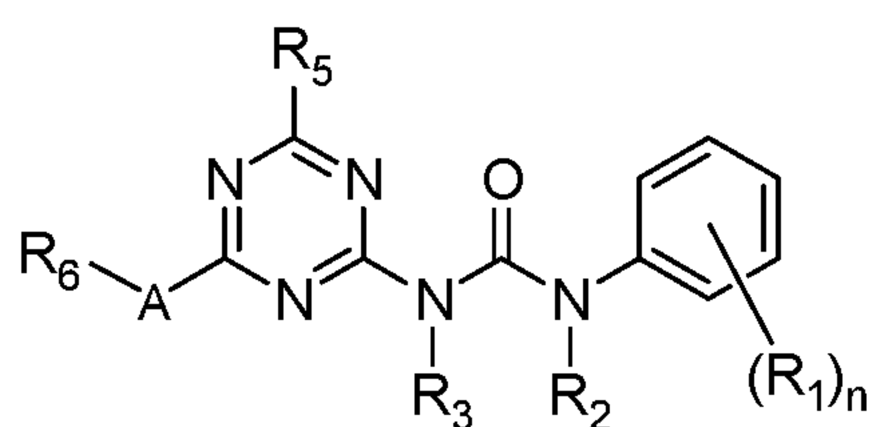
Formula (V);
