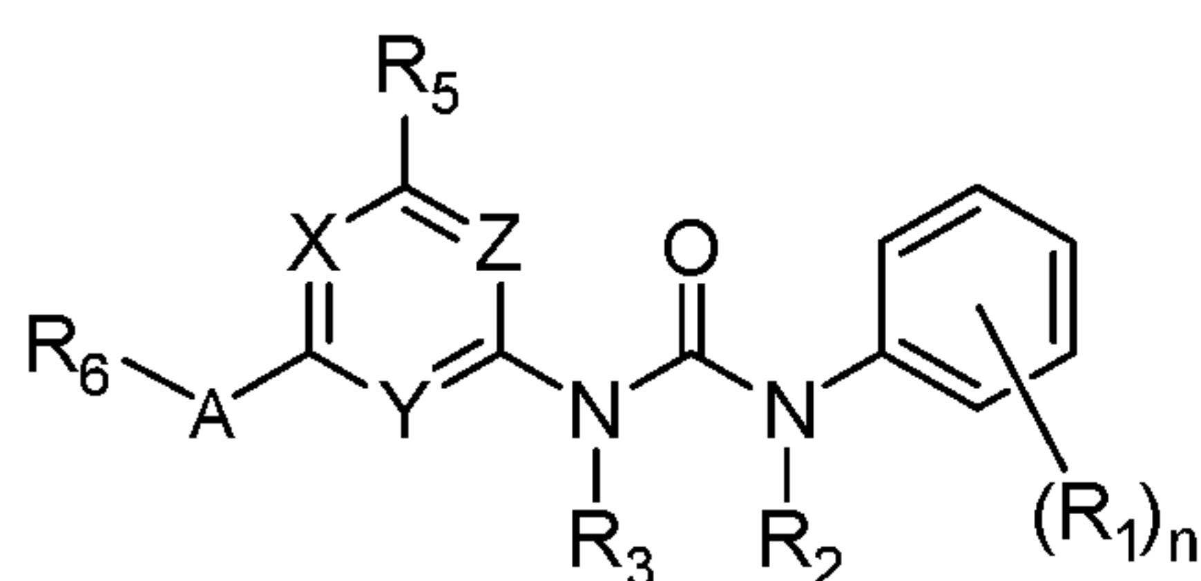
Formula (I);
