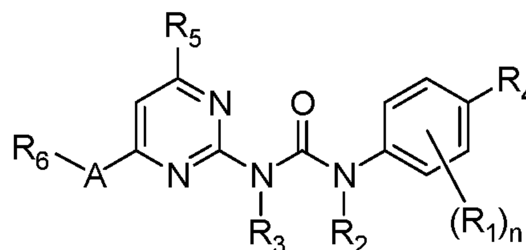
Formula (IID');
