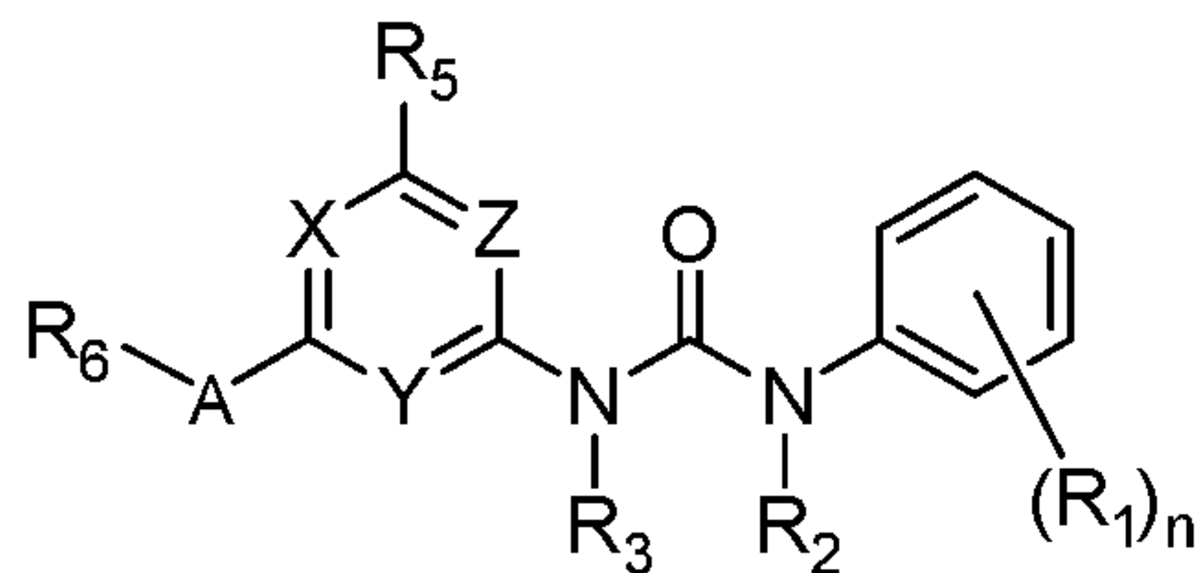
Formula (I);
