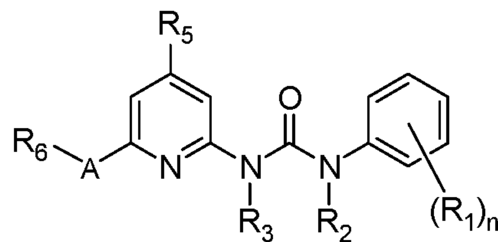
Formula (III);
