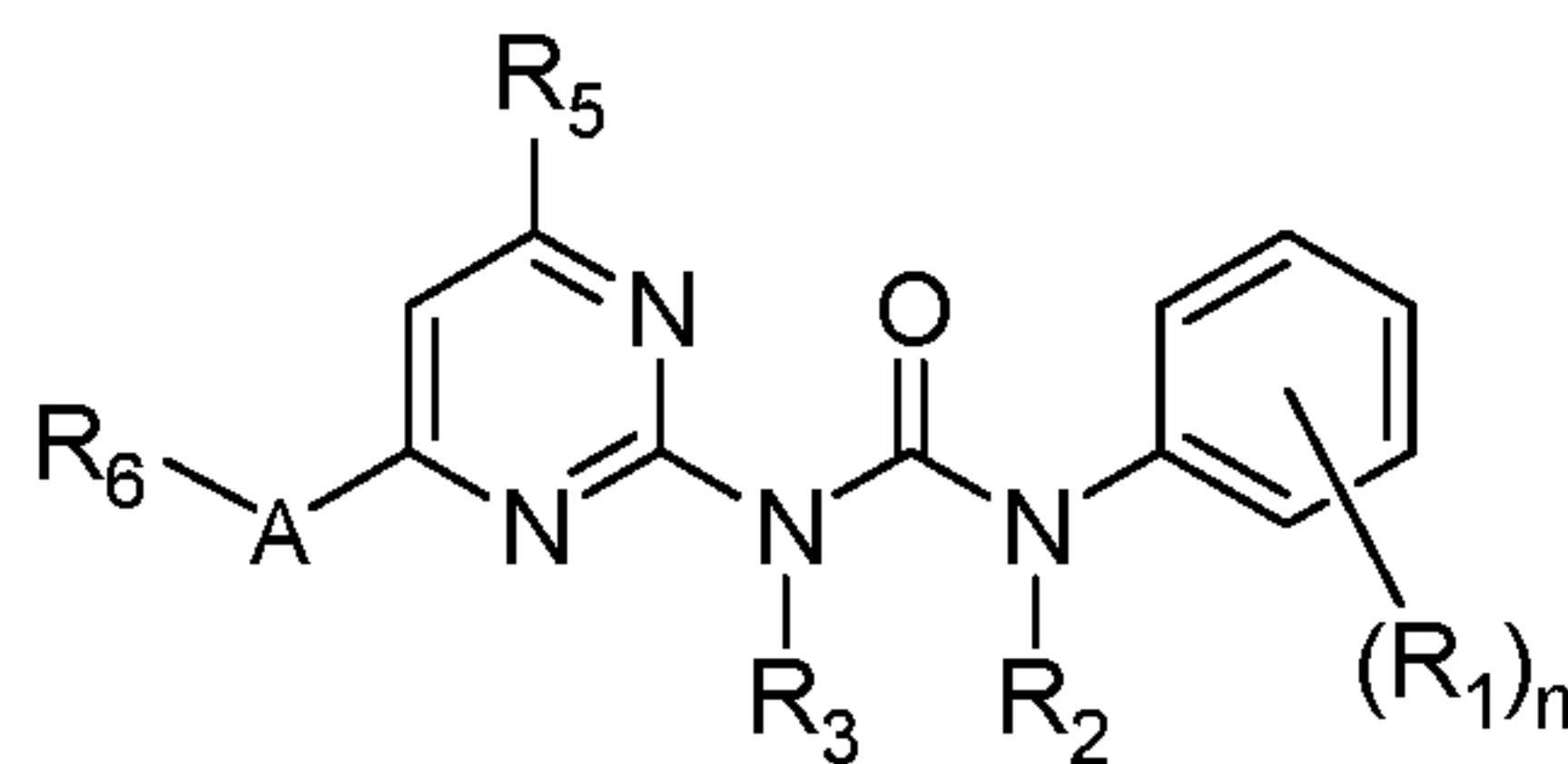
Formula (IIC);
