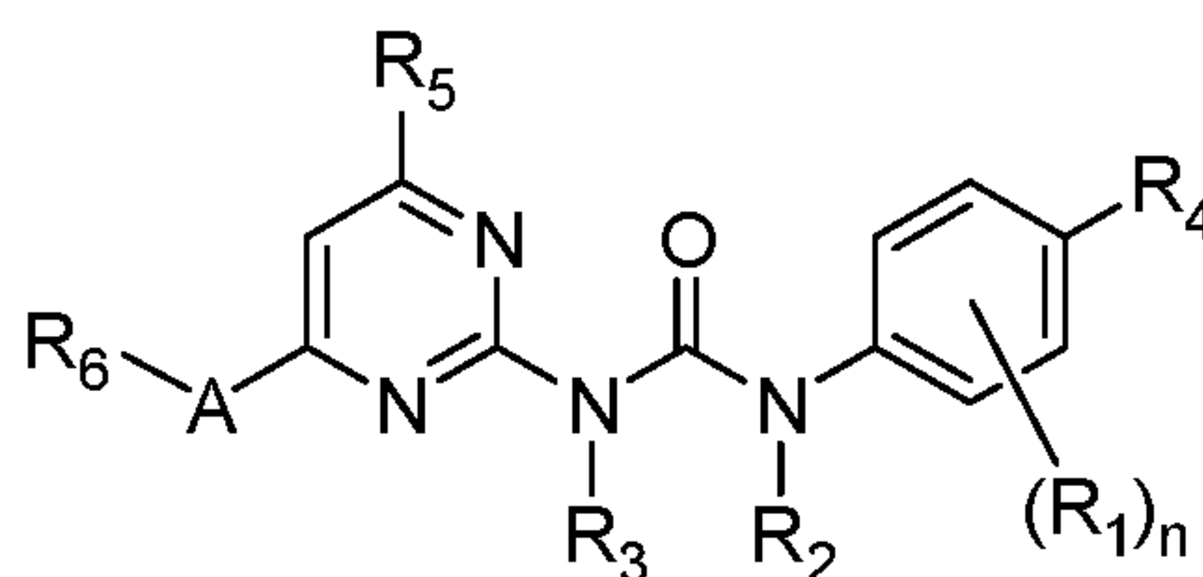
Formula (IID);
