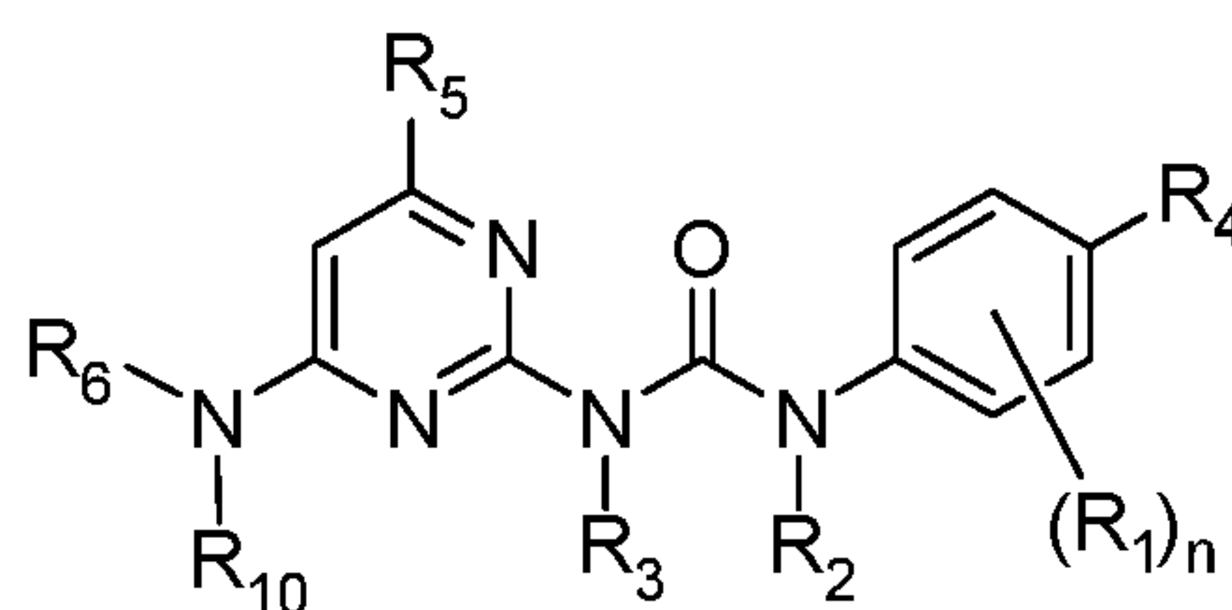
Formula (IIA');
