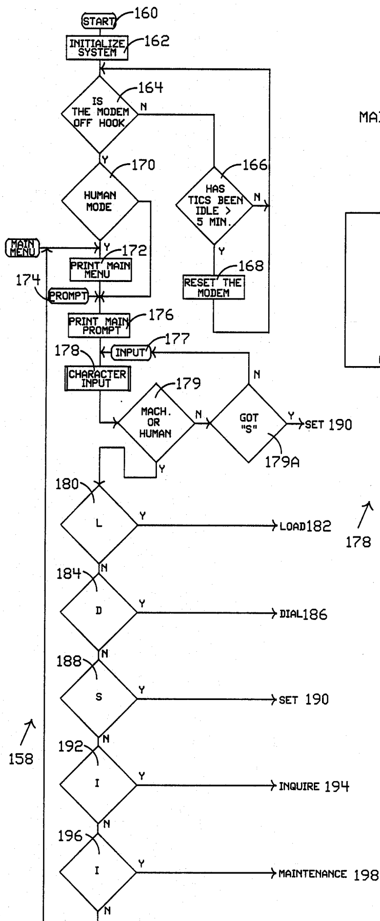
FIG - 7A
