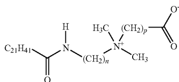
Surfactant in BET-E-40 (when n=3 and p=1 )
